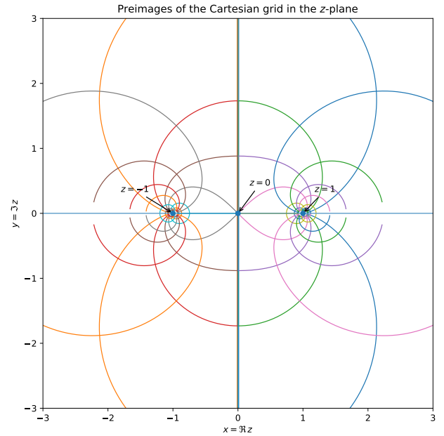
Figure 4: The hidden Cartesian grid. Vertical lines u = \Re \Gamma = \text{constant} and horizontal lines w = \Im \Gamma = \text{constant} form an ordinary Cartesian coordinate grid in the right half of the \Gamma -plane. Their local preimages under \Gamma(z) = (1 - z^2)^{-1/2} are the apparently complicated curvilinear level sets shown in the z -plane; equivalently, these curves are obtained locally by applying the inverse branch z = \pm \sqrt{1 - \Gamma^{-2}} to the grid lines. Away from critical and branch points the map is locally conformal, so the orthogonality of the Cartesian grid is preserved.
