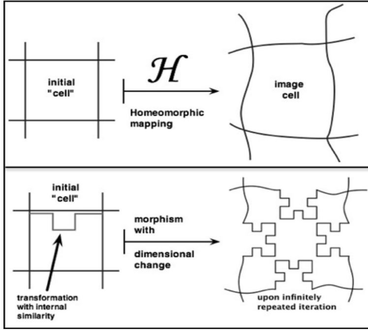
Figure 2: The continuity of homeomorphic mappings of structures is broken if once a deformation involves an iterated transformation with internal self-similarity, which involves a change in the dimension of the mapped structure. The first two or three steps of the iteration are sketched with basically the new figure jumping from (D) to approximately (D+1.45). The mediator of transformations is provided in all cases by empty set units.
