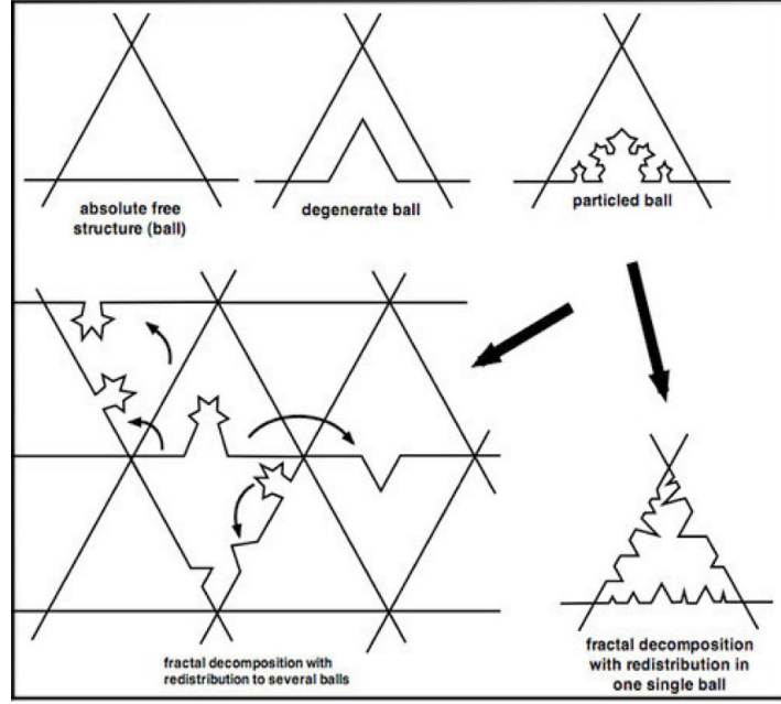
Figure 3: Scheme of the possible distribution of volumetric fractals from the particled ball.
