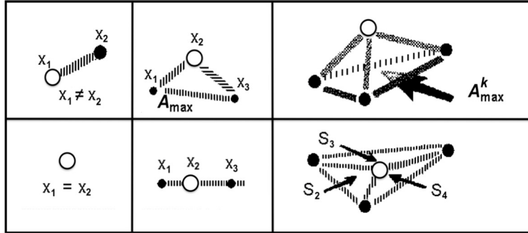
Figure 1: The first three steps of the N -angular strict inequality for the assessment of the dimensionality of a simplex. In the lower right picture, the larger side standing for A_{\max}^k is S_1 , such that in a 2D space we have exactly: S_1 = S_2 + S_3 + S_4 .
