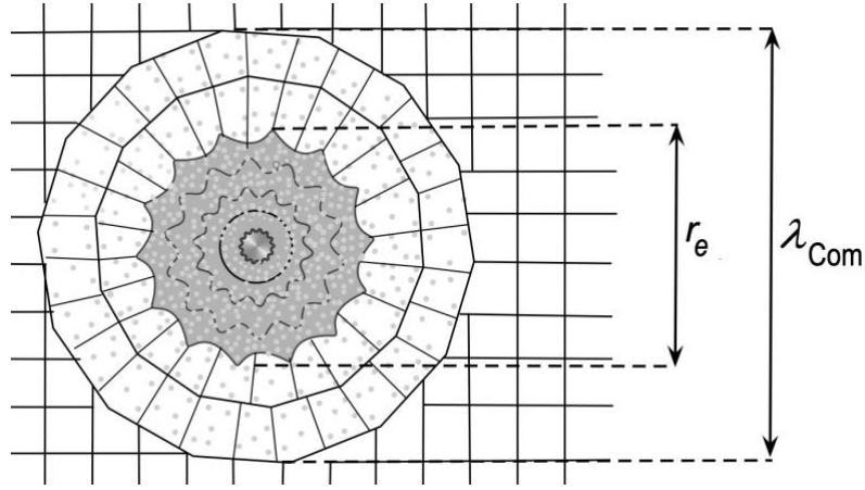
Figure 1. Deformation coat emerges in space around the created elementary particle (more details in the text below). The deformation coat consists of the inertial sub-coat initiated by the mass m , which is depicted by the diameter \lambda_{\text{Com}} (Compton wavelength), and the electrical sub-coat launched by the charge e , which is illustrated by the diameter r_e (e.g., J. J. Thomson's classical radius of electron).
