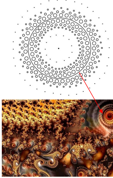
The planet as an accumulation of particles
