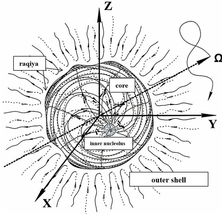
Fig. 4. A fully geometrized model of a convex stable spherical vacuum formation (in particular, a planetary Pe_y^+ -''quark 10 '')
