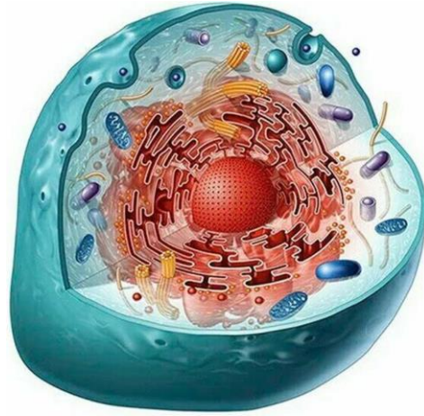
Fig. 7. Biological cell
