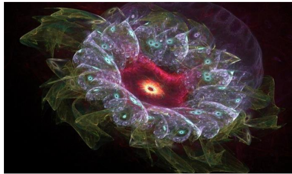
Fig. 8. Fractal illustration of the attraction of many pico-, nano- and microscopic "particles" to the core of a naked "planet" by means of the mechanism of inter-"planetary" gravity
