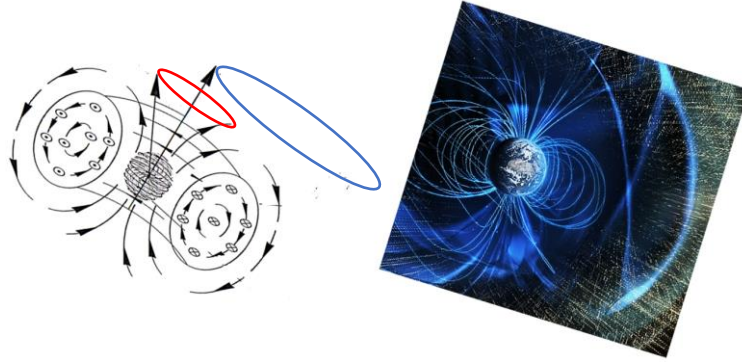
Fig. 11. Schematic representation of subcont-antisubcont currents determining the lines of force of the geometrized magnetic field of a moving neutral valence naked P_k -“planet”
