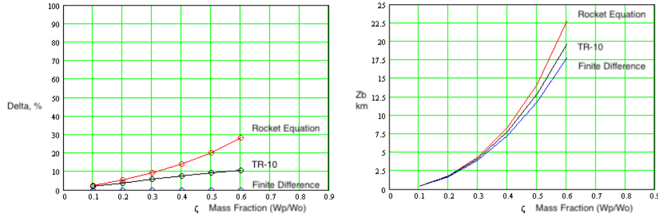
Figure-5, Large rocket (Model-2) burnout altitude (km) accuracy in percent (%) for the rocket equation and TR-10 methods normalized by the finite difference method verses mass fraction, \zeta
