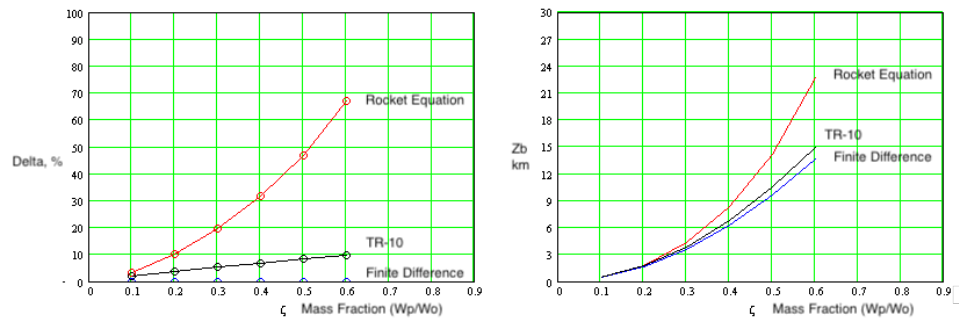
Figure-3, Small rocket (Model-1) burnout altitude (km) accuracy in percent (%) for the rocket equation and TR-10 methods normalized by the finite difference method verses mass fraction, \zeta
