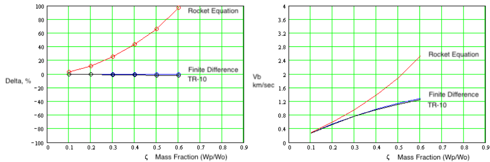
Figure-2, Small rocket (Model-1) burnout velocity (km/sec) accuracy in percent (%) for the rocket equation and TR-10 methods normalized by the finite difference method verses mass fraction, \zeta
