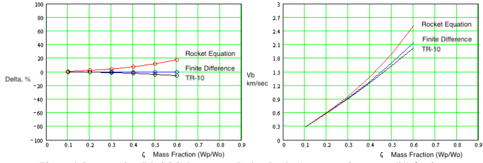
Figure-4, Large rocket (Model-2) burnout velocity (km/sec) accuracy in percent (%) for the rocket equation and TR-10 methods normalized by the finite difference method verses mass fraction, \zeta
