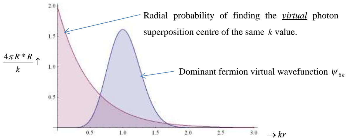
Figure 3.4. 1 Radial probabilities of \psi_{6k} and the exponential decay with radius of a virtual photon of the same k value R^*R \propto 2ke^{-2kr} . These curves look the same for all k , applying equally to virtual photons, gravitons and to large k value gluons etc.
