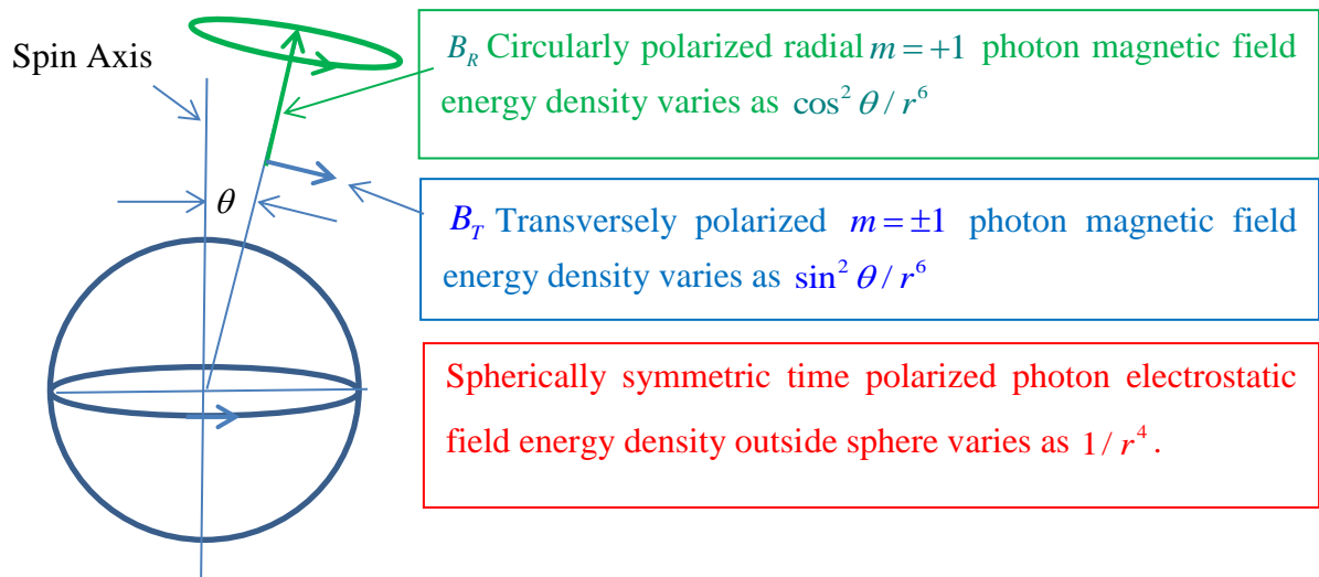
Figure 7.1. 1 Spinning electrically charged sphere. At same radius B_R @ (\theta = 0) = 2B_T @ (\theta = \pi / 2) .
