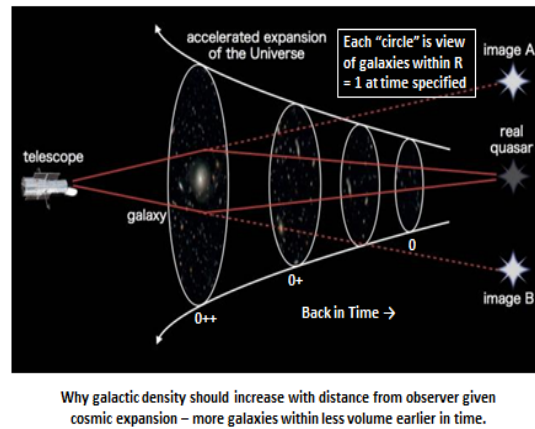
FIGURE 2. Illustration of Observable Universe as a Function of Time Given Expansion [8]
