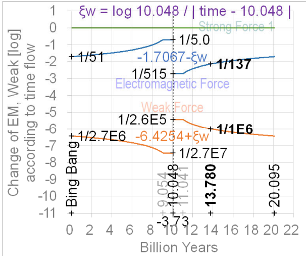
(a) Electromagnetic and Weak forces
