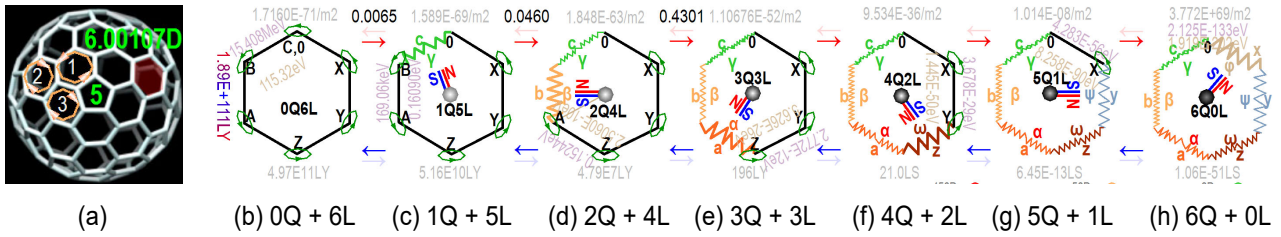
Fig. 21 Change of six dimensional universe
