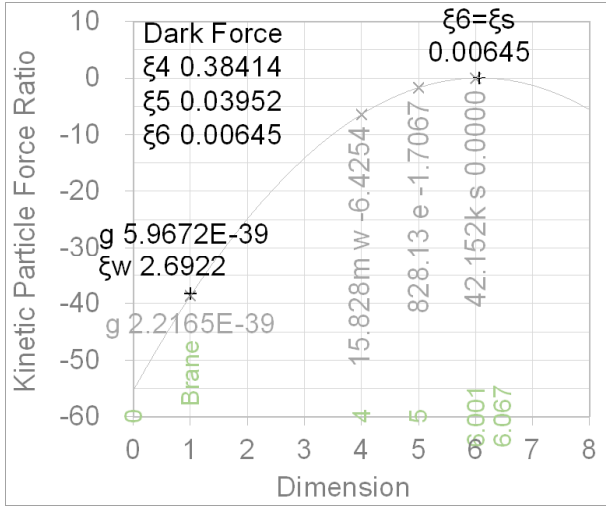
(a) Particle force mass
