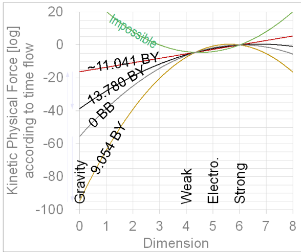
Fig. 23 Constraint condition of Four Forces
