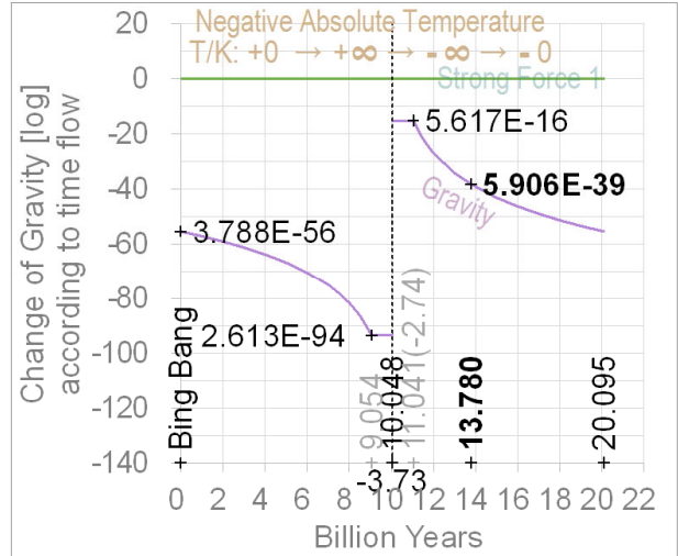
(b) Gravitational force
