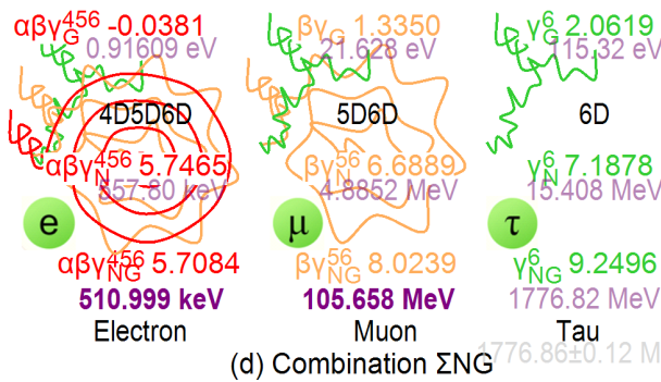
Fig. 3 Particle shape and log-mass
