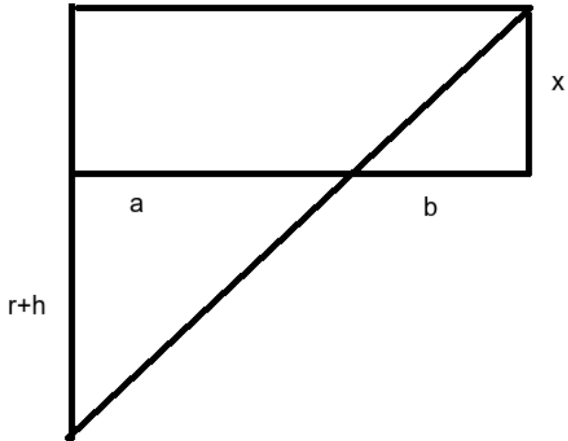
Graph3: the geometric connection between different lift-sizes to calculate length a resp. b by proportional lengths at the same angle.
