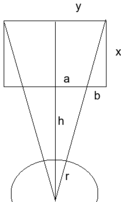
Graph 1: Einstein-Lift above earth with three radial gravity field-lines in a height of h = 100 \text{ km} . (No scaling but only qualitative drawings.)
