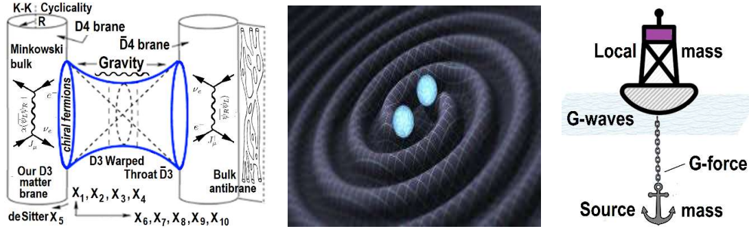
Figure 1. a) M-theoretic brane concept of the origin of gravity in the XD bulk. b) Depiction of LIGO G-wave colliding black holes. Fig. courtesy NASA/C Henze [11]. c) Machian-Vigier inertial G-model, where inertial flux (source mass) is cosmological – Earth, sun, galaxy.
