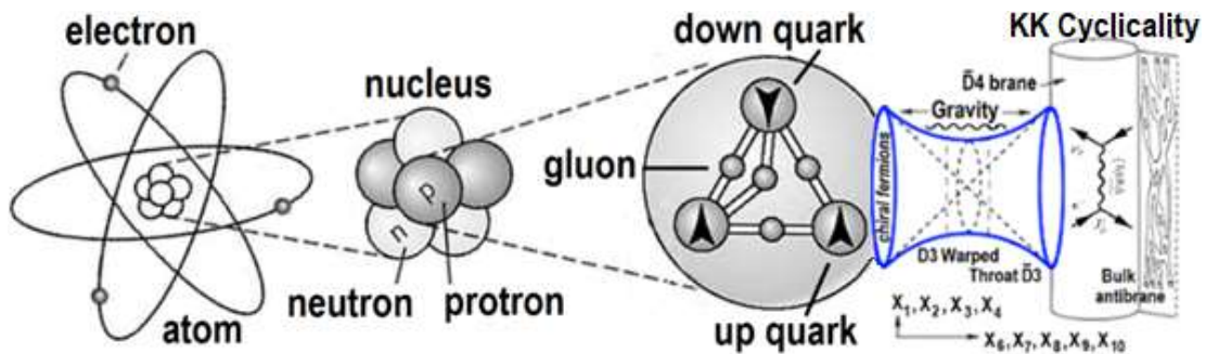
Figure 6. Unified field – M-theoretic model of matter. Atom → nucleus → quarks on a D3 brane (Fig. 1a-left cylinder). At the semi-quantum limit tunneling occurs through an XD warped throat to the antispacetime \bar{D}3 brane bulk with LSXD brane topology.
