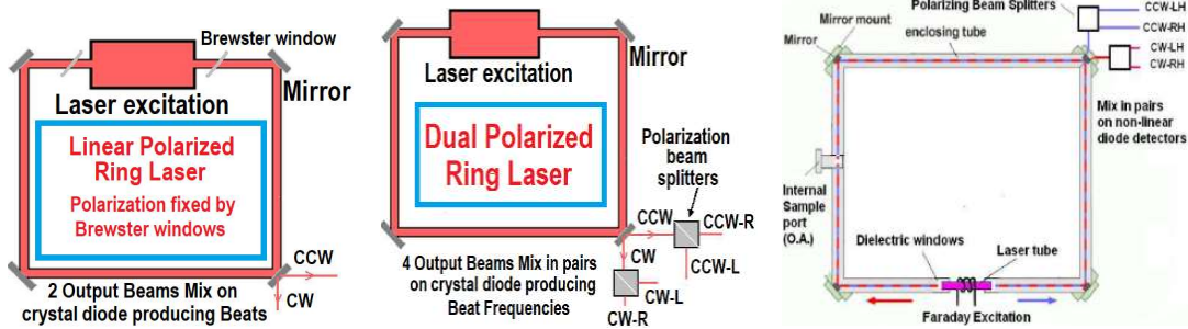
Figure 4. a) 2 beam (CW – CCW linearly polarized) Sagnac Ring with internal laser source. b) 4 Polarized beams – CWLH, CCWLH, CWRH, CCWRH Sagnac Ring with internal laser source. c) Modern dual polarized Ring Laser design. Figures adapted from [6-8].
