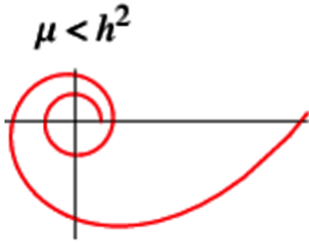
Figure 4: Spiral shape called "Cotes's Spiral." for \mu < h^2 . [24, 25]
