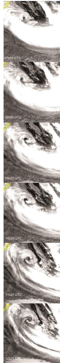
Figure 3: Image of the “bomb cyclone” moving to the Atlantic Ocean. Image in the infrared spectrum, July 1, 2020, for the 5 hour time slot, from 07:20 to 12:20 UTC, REDEMET. (Adapted) [23].
