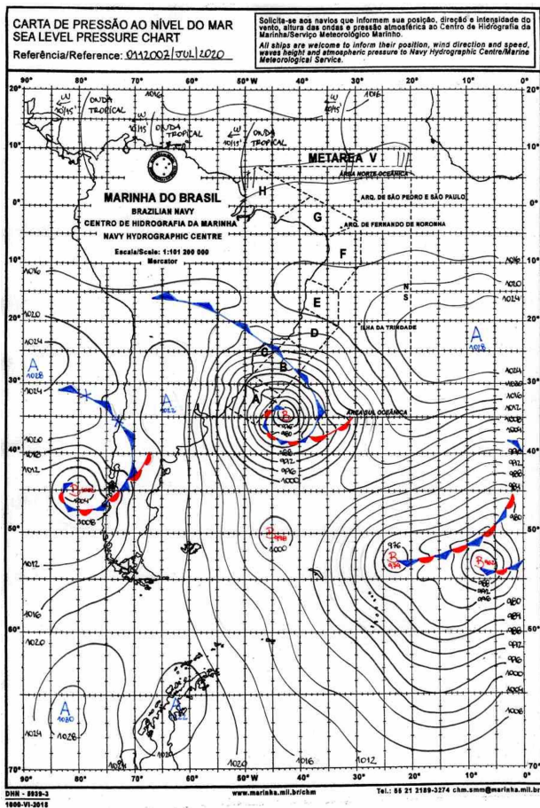
Figure 2: Synoptic Letters, from July 1, 2020, at 12h00 UTC. Navy Hydrography Center. Brazil's navy. Synoptic Letters. [22]
