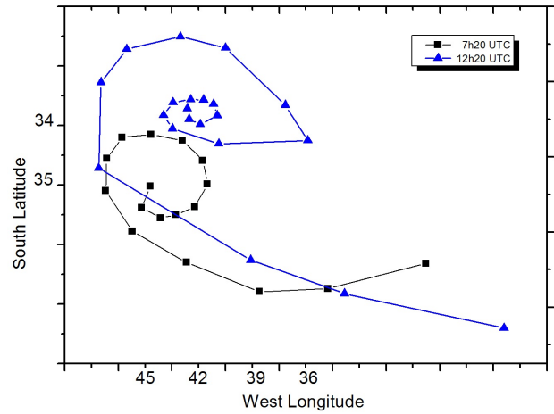
Figure 5: It represents the coordinates of the points collected from Figure (3), in Longitude and Latitude, using the Isobaric found in Figures (1) and (2). [Authors]
