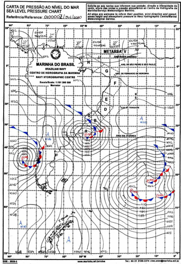
Figure 1: Synoptic Letters, from July 1, 2020, at 00h00 UTC. Navy Hydrography Center. Brazil's navy. Synoptic Letters. [22]
