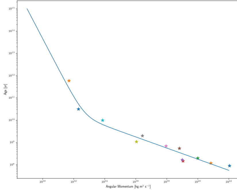
Figure 3: Angular momenta and ages of celestial bodies, as given by Stellar Metamorphosis, with reproduced fit. [4]
