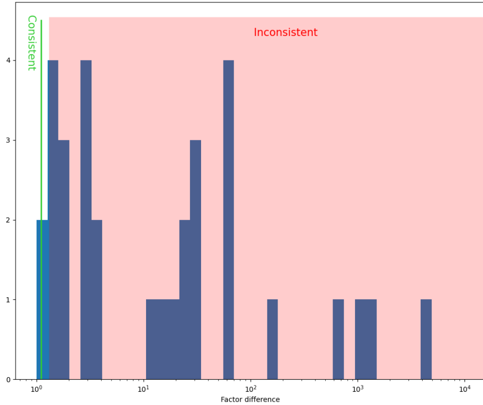
Figure 5: Histogram of all analyzed factor differences. Factor differences are equal to 1 when two methods of age estimation are consistent with one another (as a factor of 1.1 characterizes two measurements that are within 10% of each other). The large majority of analyzed methods from Stellar Metamorphosis are severely inconsistent, with factors of > 1,000 , indicating age discrepancies of > 100,000\% .
