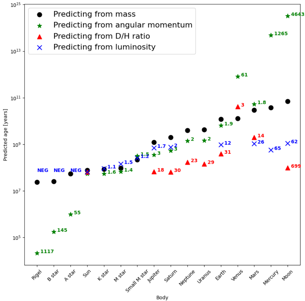
Figure 4: Diagram showing ages given by Stellar Metamorphosis for Solar System and other bodies. For each method, the difference between the mass prediction and each of the other prediction methods is given as a factor difference, which is defined as the ratio of the age prediction for the method in question by the WT diagram predictions. (If the ratio is < 1 , then the reciprocal is quoted.) Note that several of the ages predicted using the body’s bolometric luminosity result in negative ages; these instances are marked as “NEG” in the plot. There is a large discrepancy in the ages of almost all of the objects. No two age predicting methods agree to any reasonable degree in nearly any case, and the methods disagree by a factor of 260, on average, across all of the methods.
