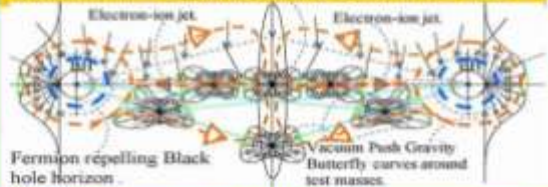
Scheme of the electric SABH principle around the sun.
