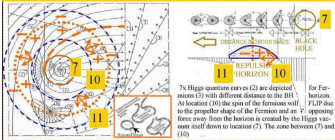
Figure 7, BH with pushing vacuum vector fields in detail.
