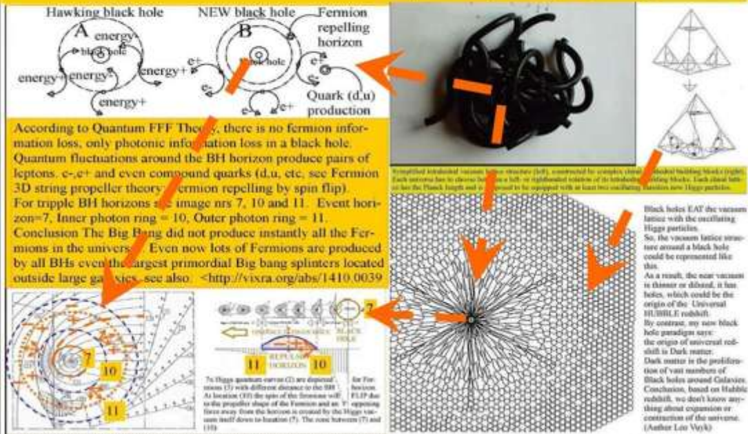
Figure 6, the new physics principle of black hole charging and vacuum diluting.
