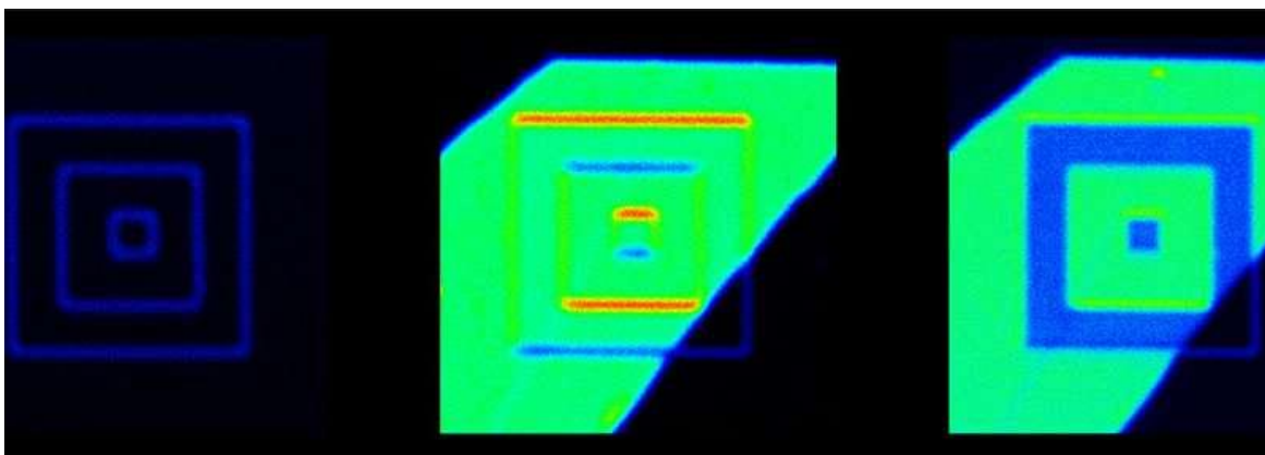
Light signals reflected from PZT (left), reflected from the molybdenum disulfide-PZT nanostructure (center), and transmitted through the nanostructure (right). The center image,
