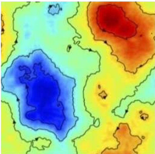
Large-scale circulating flows at scales much larger than the characteristic size of the underlying pattern of vortices. Credit: University of Barcelona
