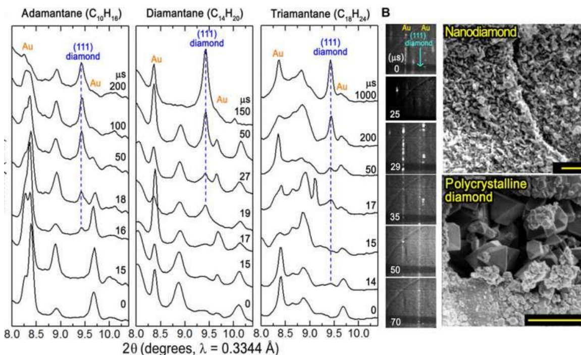
Onset timing of diamond formation from lower diamondoids. (A) In situ XRD patterns of three diamondoids as a function of increasing laser-heating duration. Nonlabeled peaks belong to the sample. (B) Cake integration of two-dimensional diffraction images highlighting the texture of diamond growth as a function of increasing laser-heating time. Representative SEM images of nanodiamond and polycrystalline diamond. Scale bars, 2 μm. Credit: Science Advances , doi: 10.1126/sciadv.aay9405
