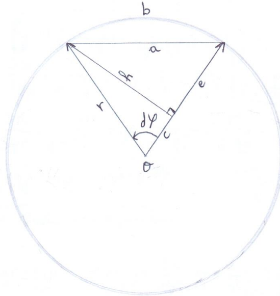
Fig.1: The trigonometric circle of radius r=1 .
