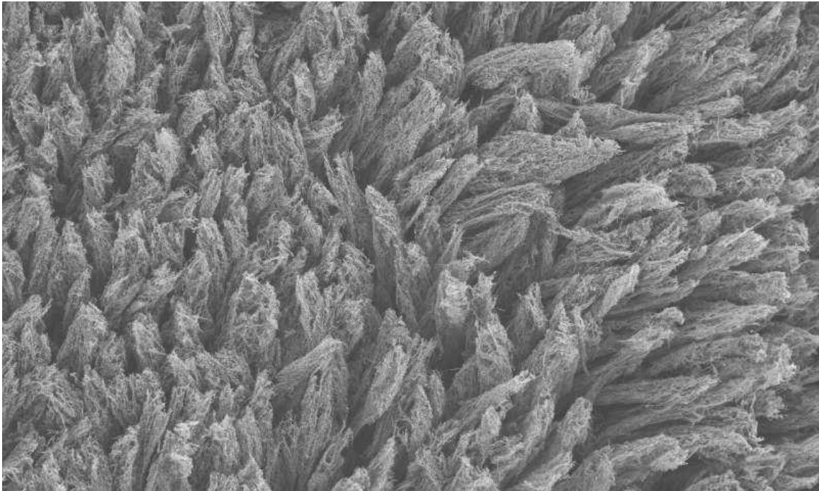
A scanning electron microscope image shows a composite of laser-induced graphene and polystyrene. Credit: Tour Group/Rice University
