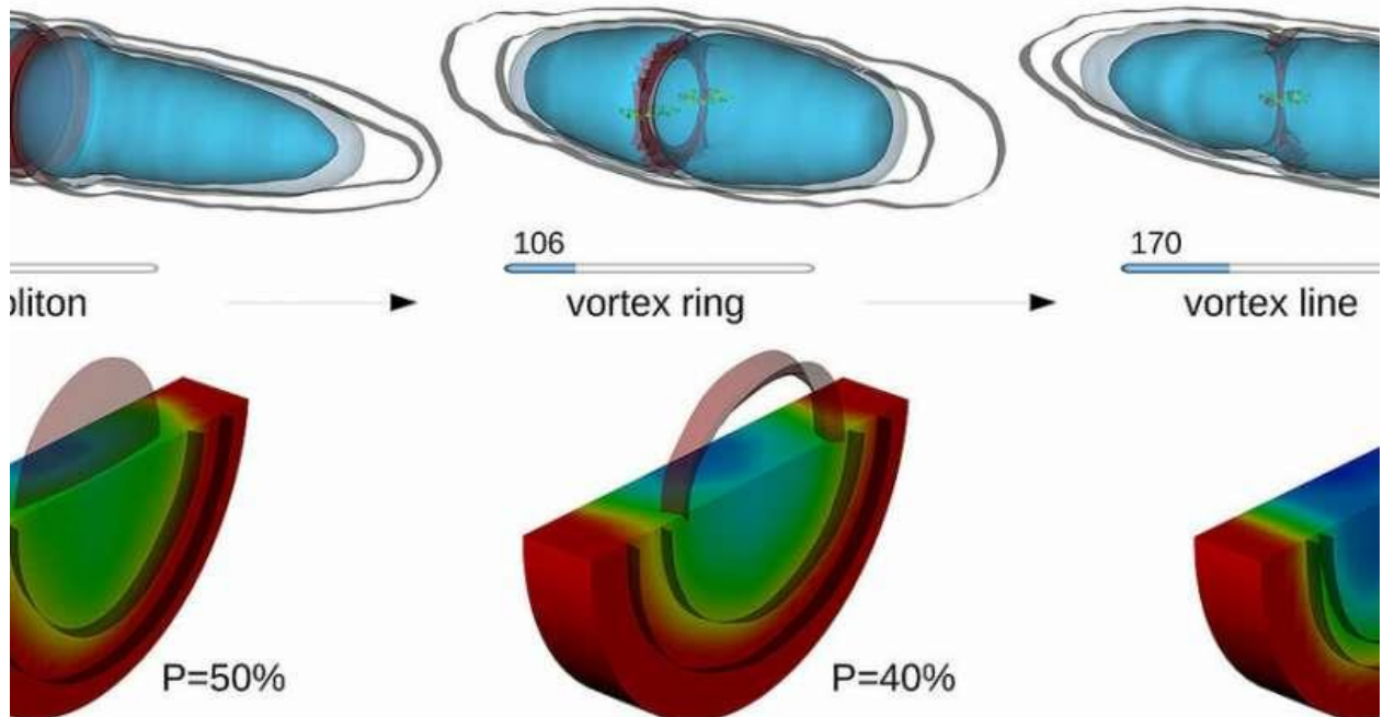
The shapes represent the various vortices that the researchers discovered forming in a spin-imbalanced atomic cloud. Credit: Gabriel Wlazłowski
