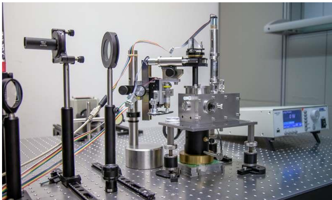
This surface force apparatus exploits light interference to resolve distances between ultrasmooth surfaces at an accuracy of 0.1 nanometers. Credit: © 2019 KAUST
