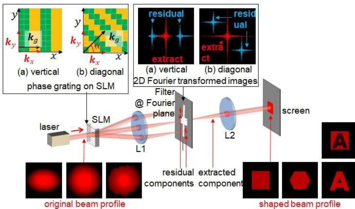
Figure 2. Experimental layout: phase grating and filtering in the Fourier plane of the 4f system. (a) vertical phase grating (conventional method), (b) virtual diagonal phase grating (new method). Credit: © 2019 Nakata Y. et al., Scientific Reports .
