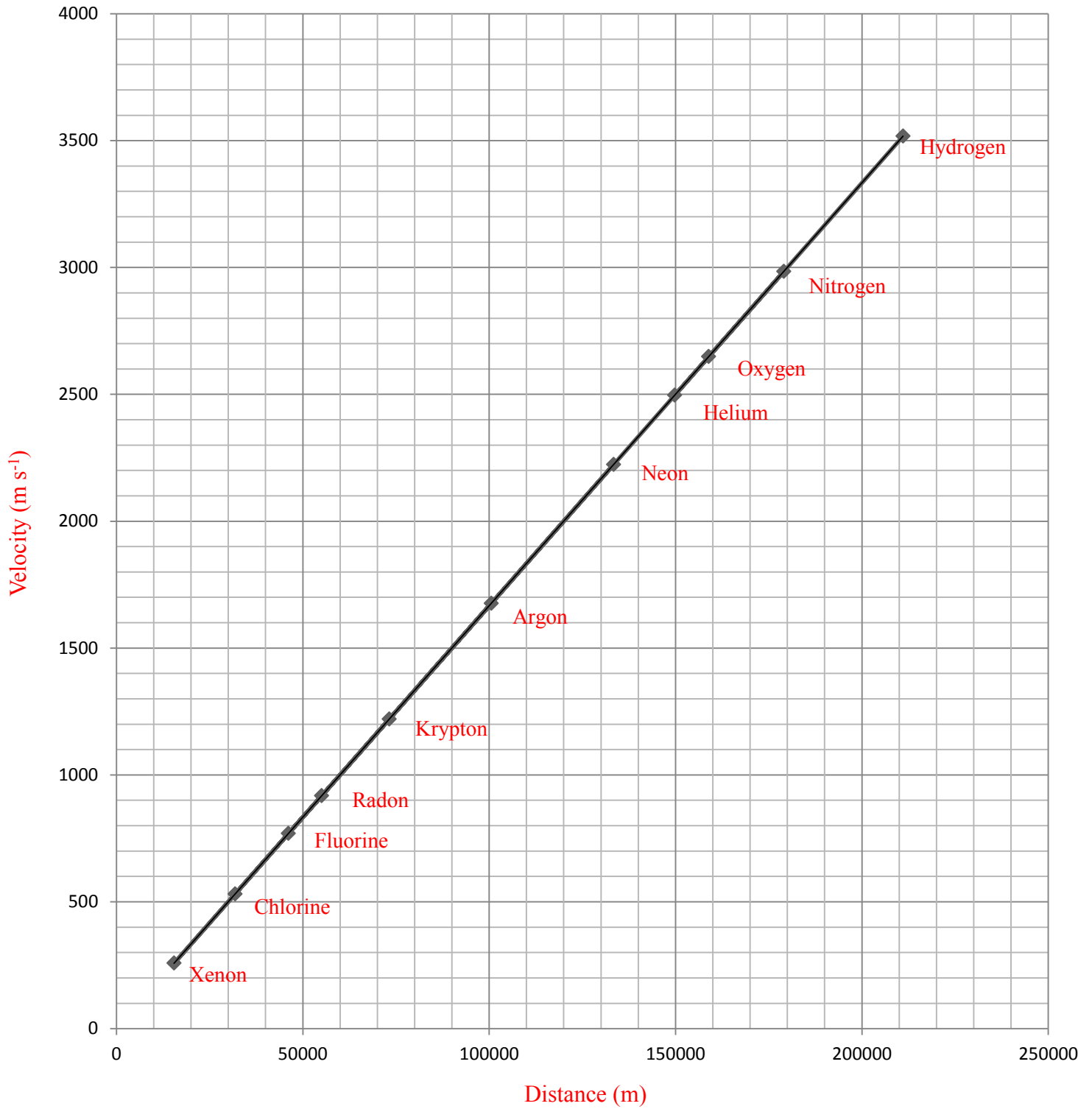
Graph 5. Velocity-distance relation plot for molecules diffusing at extreme random temperature. Observation time = 60 seconds ( Table 6 ) (Slope = 0.016666666 m s -1 m -1 )
