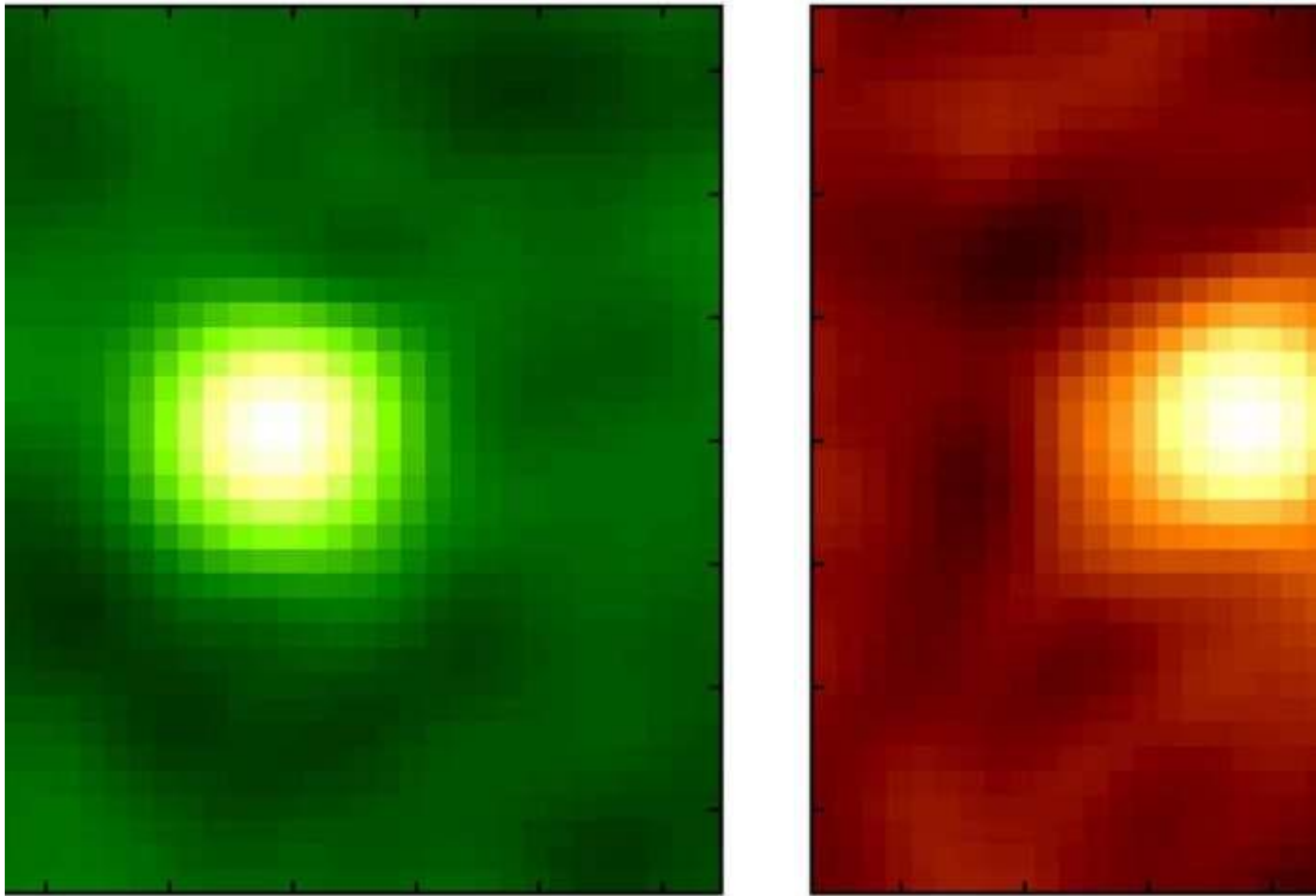
Figure 2: Emission from carbon monoxide (left) and cold dust (right) in WISE1029 observed by ALMA. The image size is 3 square arcsecond. Credit: ALMA (ESO/NAOJ/NRAO), Toba et al
