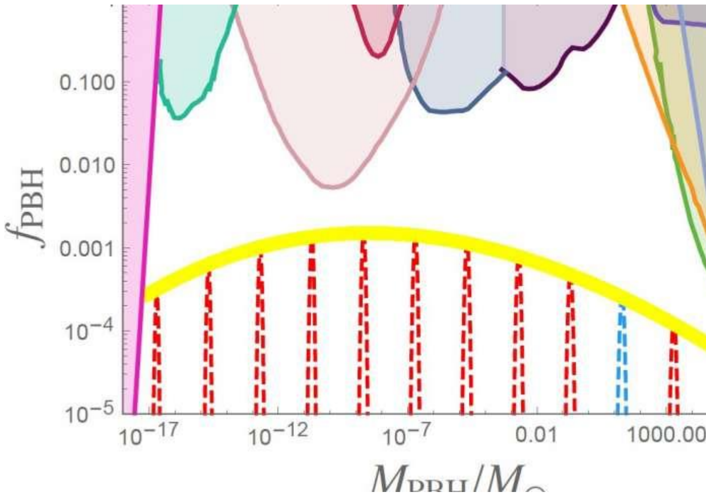
This figure shows the fraction of dark matter due to primordial black holes (vertical axis), as a function of their individual mass in solar masses (horizontal axis). The shaded areas are excluded by astronomical observations. The resonance ...more
