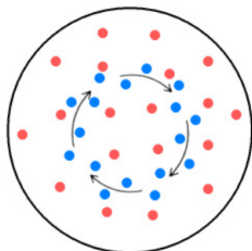
Burchell's image of electrons circling in a disk, with internal magnetic attraction
