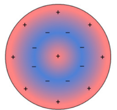
Burchell's image of magnetic attraction and repulsion of circling electrons leaving positive and negative regions within a disk
