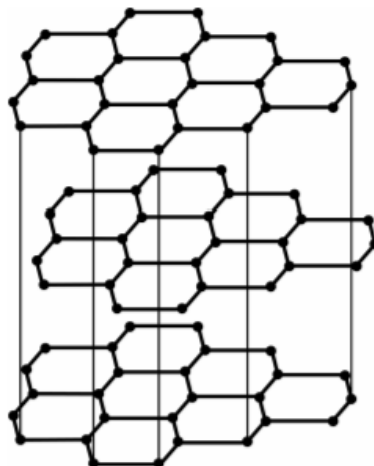
FIGURE 6. Schematic representation of the layered lattice of graphite, proposed to be the most energetically favorable crystalline form of metallic hydrogen
