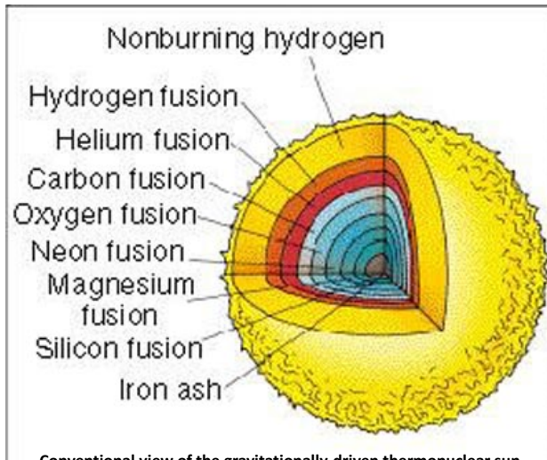
Conventional view of the gravitationally-driven thermonuclear sun (from Chaisson & McMillan, Astronomy Today, http://ircamera.as.arizona.edu/NatSci102/NatSci102/lectures/starevolution.htm )
