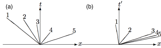
Figure 3: Worldlines of free particles, when (a) observed in a frame at rest, and (b) observed in a moving frame. Numbers over the worldlines are used to identify the particles.
