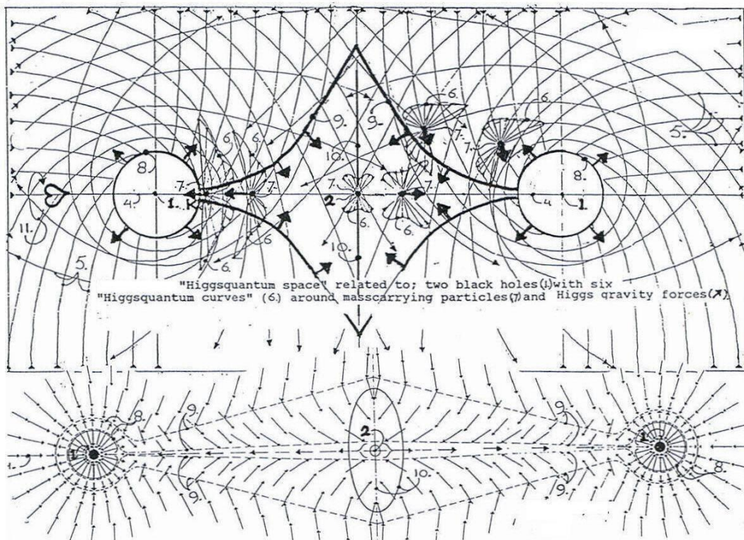
Figure 4, Axion Higgs Vacuum structure around a set of two Black holes, as is found to be present around Planetary nebula and early Galaxies and Herbig Haro objects.
