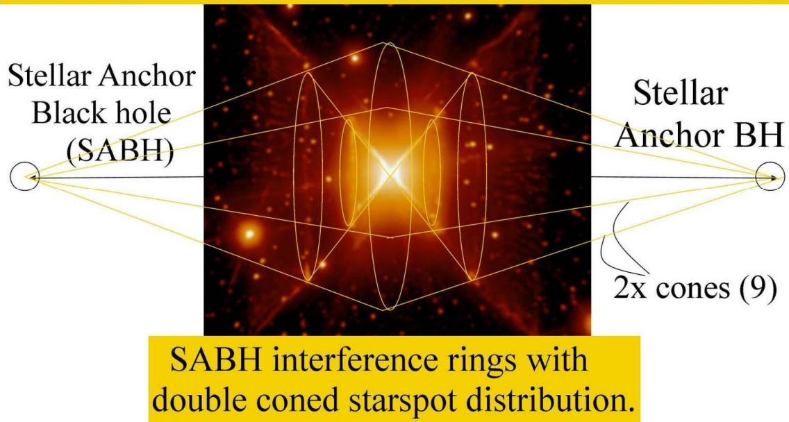
Figure 3, The Red Square Planetary nebula MWC922, equipped with double cone structure of expelled material including trailing starspots (Micro Black Holes). There are FOUR cones of interferences originated by the two Stellar Anchor black holes (SABHs). These four cones seem to interfere with the TWO cones of expelled material of the star, leading to FOUR rings of interference.
