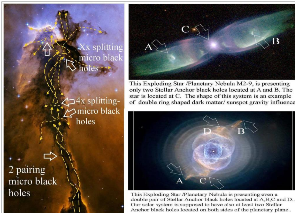
Figure 6, The Spire Eagle nebula, with two Planetary nebula, examples of the importance of black holes in the universe.
