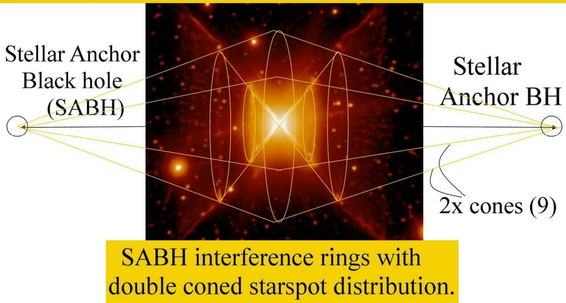
Figure 3, The Red Square Planetary nebula MWC922, equipped with double cone structure of expelled material including trailing starspots (Micro Black Holes). There are FOUR cones (figure 4) of interferences originated by the two Stellar Anchor black holes (SABHs). These four cones seem to interfere with the TWO cones of expelled material of the star, leading to FOUR rings of interference.
