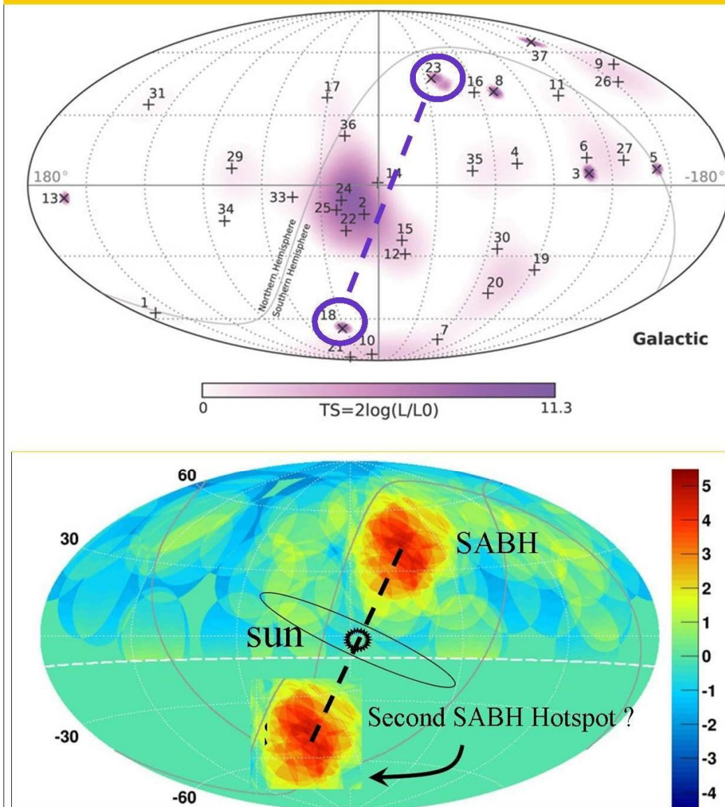
Figure: 8, 9-july 2014. first evidence for the first Solar Anchor Black Hole. (SABH) A hotspot with powerful cosmic rays found under the Big Dipper, by the University of Utah. Now ( 2017) however the southern counterpart ( the second SABH hotspot) is found, see figure 1.
