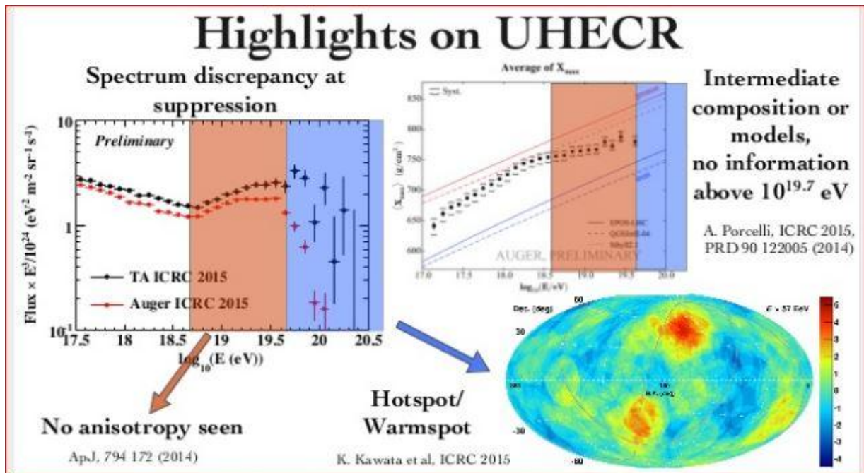
Figure 2, UHECR = Ultra High Energy Cosmic Radiation
