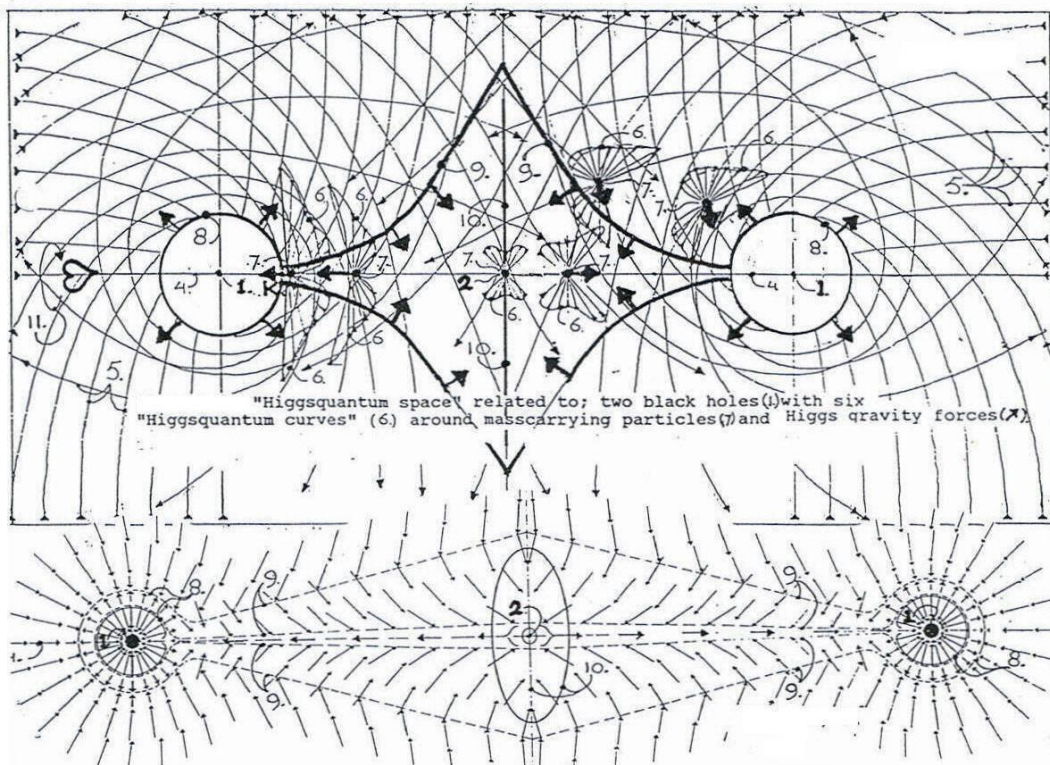
Figure 4, Higgs Vacuum structure around a set of two Black holes, as is found to be present around Planetary nebula and early Galaxies and Herbig Haro objects.
