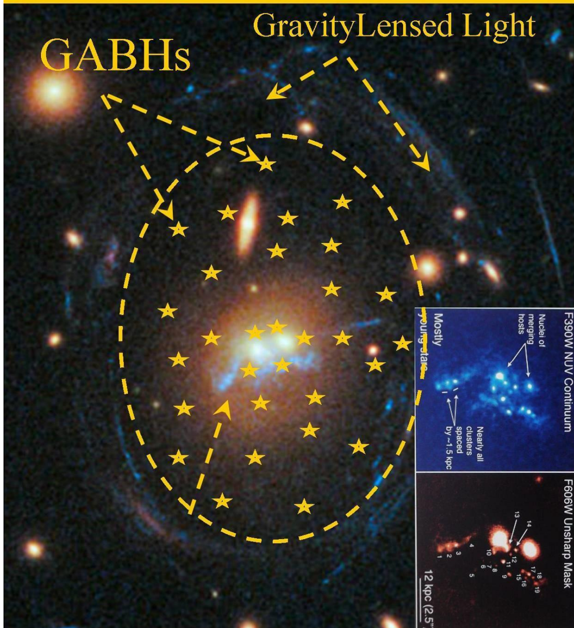
Figure: 9, Gravity lensed light through central hole in the globular Shell of Dark matter Black Holes or Galaxy Anchor Black Holes ( GABHs). The absence of GABHs in the centre is supposed to do the job.
