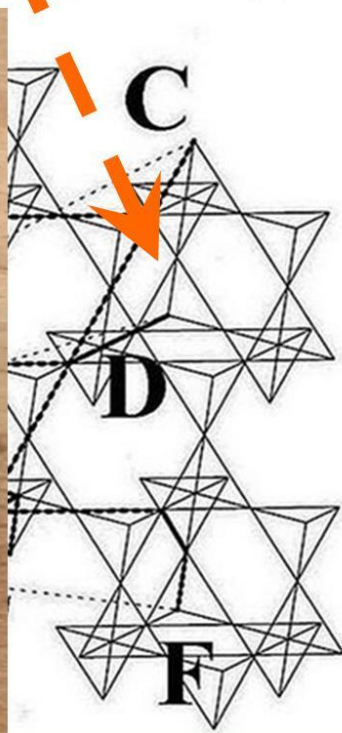
Figure 2, A stable black hole nucleus is large enough to “eat” the vacuum particles and grow by it.
