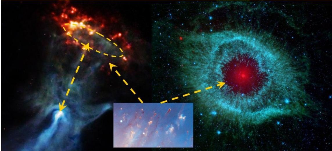
Figure 3, The A-symmetric B 1509-58 nebula , and symmetric Helix nebula as examples of the difference between Fermion and Black hole Quantum Gravity effects.
