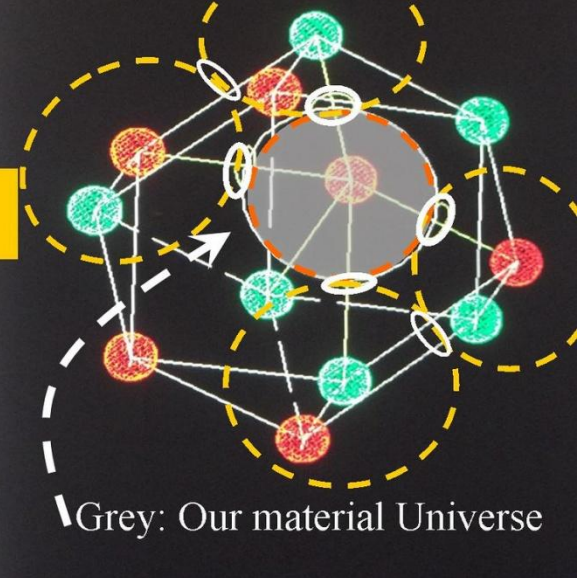
Figure 15, Our position in a 8 or even 12 fold multiverse based on fluctuation anomalies (universal contact areas)
