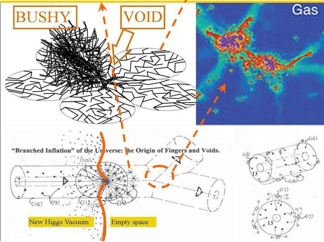
Figure 10 , BBBH , the Big Bang Black Hole splintering into smaller BHs and evaporating into the oscillating Axion Higgs Vacuum lattice .
