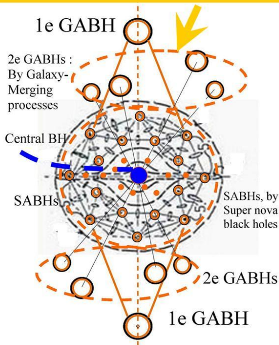
Figure 5, Merging galaxies with external GABHs (Galaxy Anchor Black Holes) observed here as dwarf globular galaxies formed around GABHs.
