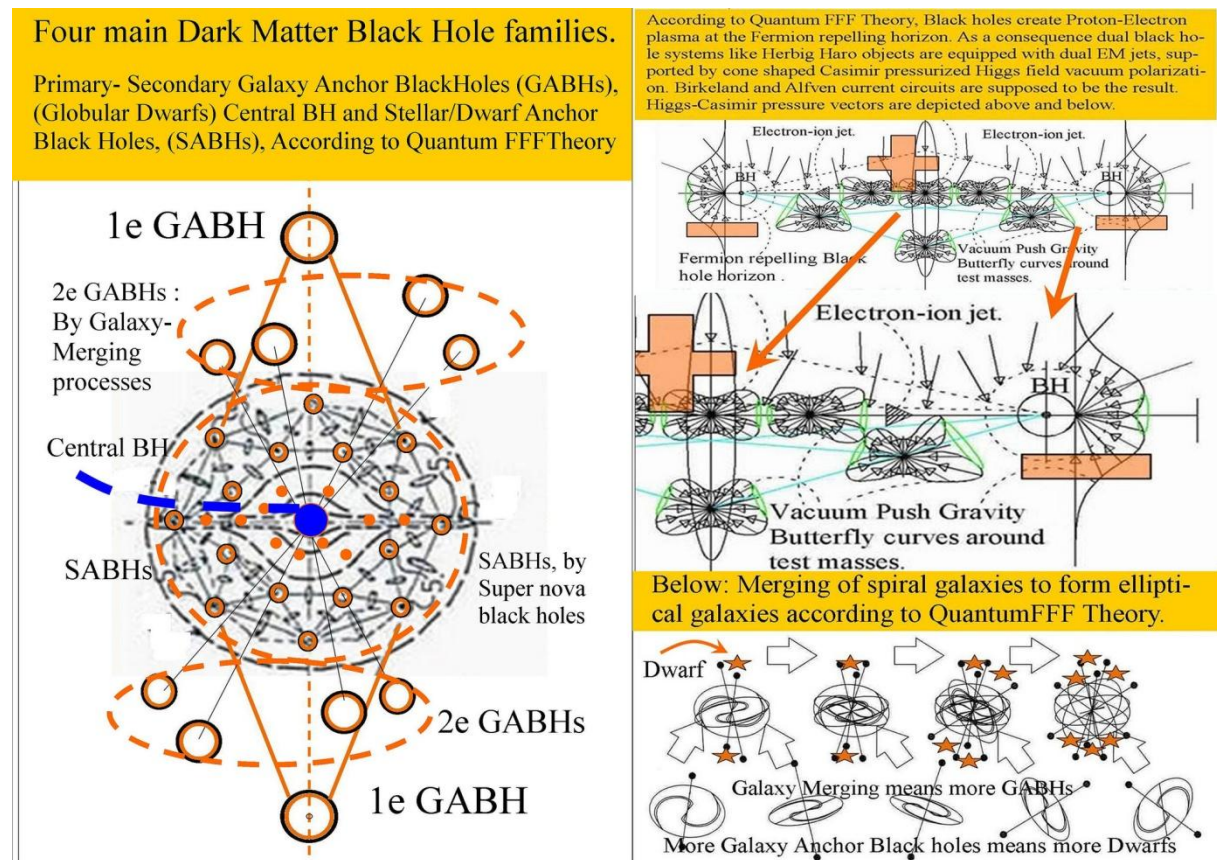
Figure 9, GABHs as the largest unit of Dark Matter black hole families
