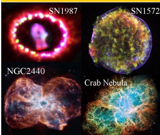
Figure 4, Other examples of Quantum Gravity effects on ejected rings of micro black hole starspots at work in different nebula .
