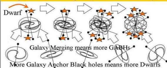
Figure 5, Merging galaxies with external GABHs (Galaxy Anchor Black Holes) observed here as dwarf globular galaxies formed around GABHs.
