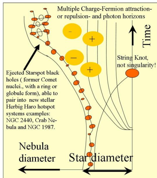
Figure 4, Other examples of Quantum Gravity effects on ejected rings of micro black hole starspots at work in different nebula .
