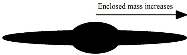
Figure 3. In case of a galaxy, the baryonic enclosed mass increases with distance from the centre of the galactic nucleus.
