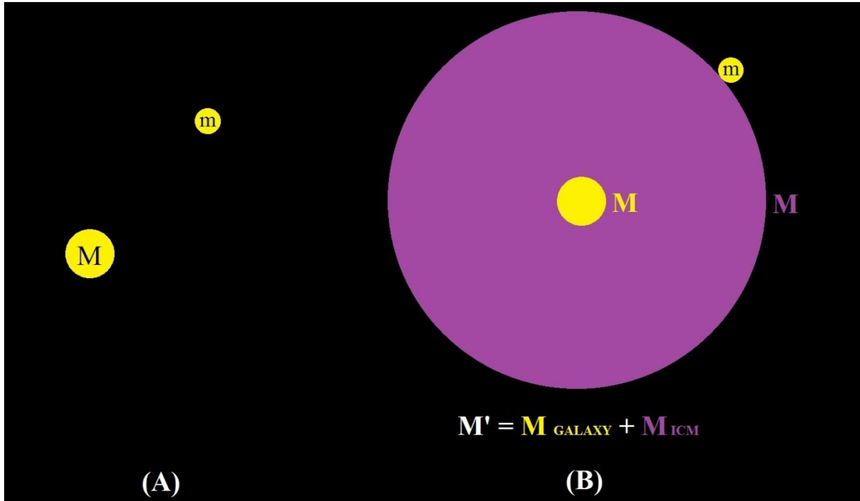
Figure 5. (A) Galaxy cluster in visible wavelength. ICM remaining invisible, the only optically visible components are M and m. The orbital and escape velocity of m is therefore expected to be with respect to the mass M, since it is the only optically visible enclosed mass. However, the orbital velocity of m is more than expected, thereby resulting into a mass discrepancy. The presence and role of ICM as enclosed mass was not known before the introduction of space-based X-ray astronomy. (B) Galaxy cluster in visible and X-ray wavelengths. The enclosed mass constituted by the central galaxy and ICM is visible. The orbital and escape velocity of m is therefore with respect to the entire enclosed mass M' , constituted by M_{\text{GALAXY}} + M_{\text{ICM}} .
