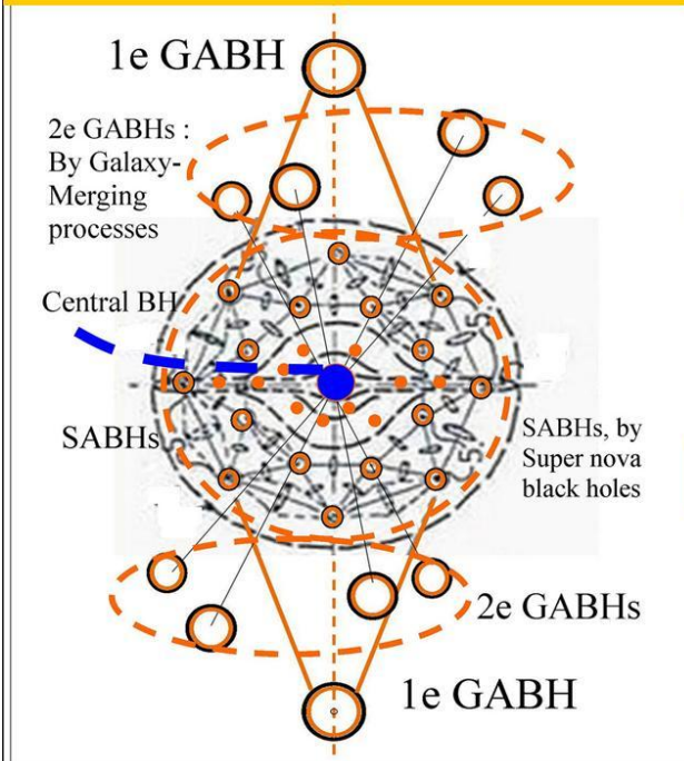
Figure 1. Simple external (new physics) black hole configuration.
