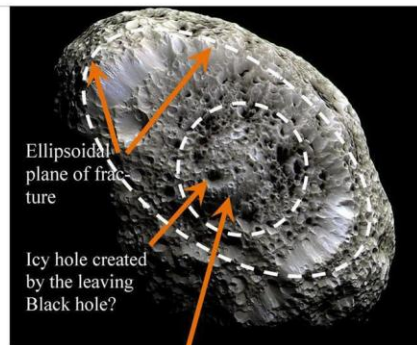
Figure 2, Principle of the new black hole paradigm All Fermions going OUT only dark energy of the oscillating Vacuum lattice frame is going IN..
