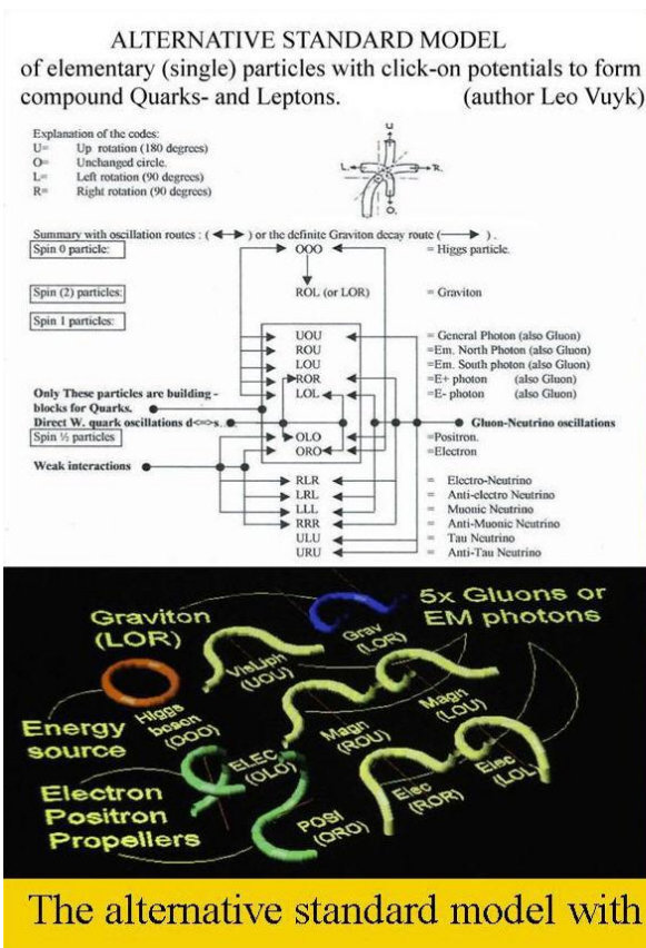
Figure 8, the alternative standard model ref. [5]
