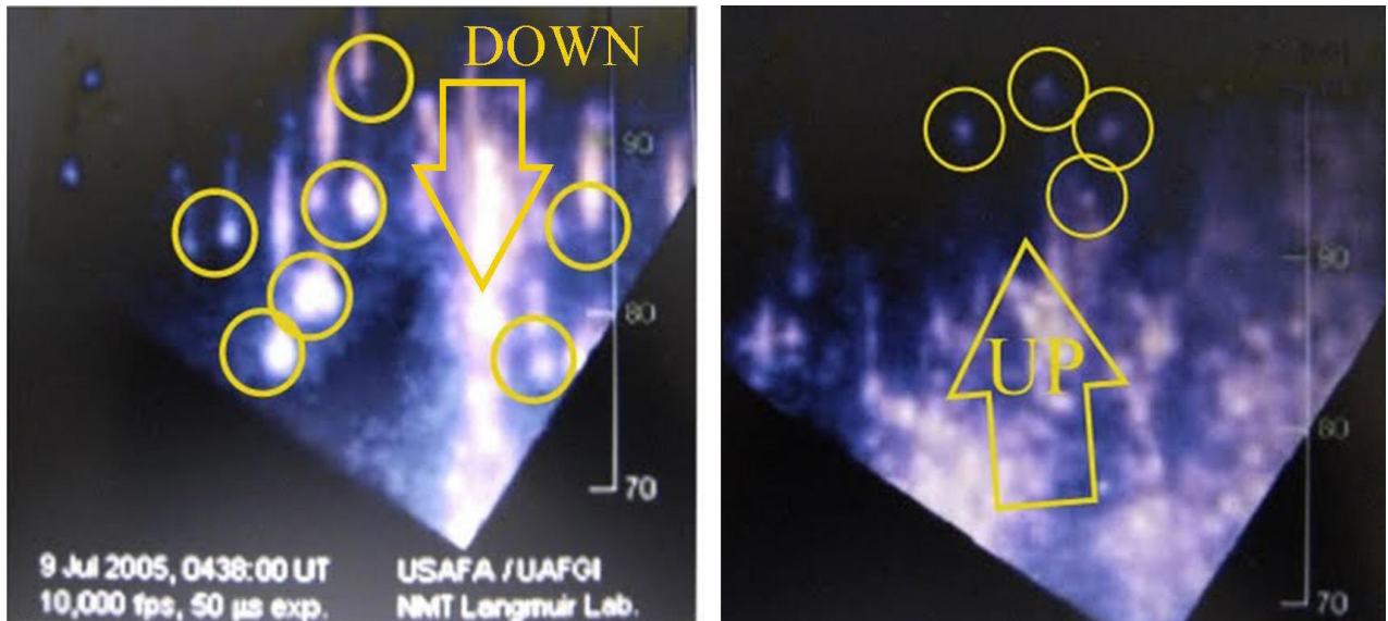
Figure 3, FIREBALL images observed inside a Sprite by a video. The video is made by a High speed camera (10.000 f/sec) of the Langmuir laboratory (USA, 2005) looking at 70-120 km altitude.
