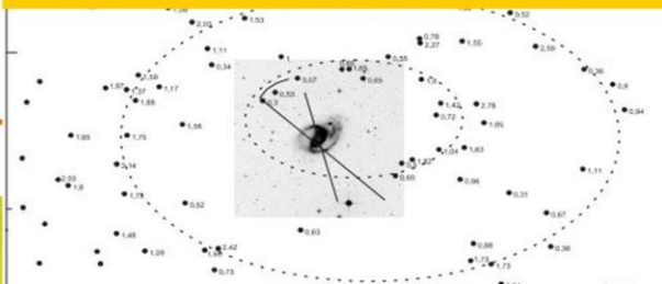
Cygnus A Radio Galaxy with dual gas producing Quasars (dual Hotspots) and growing black hole based galaxy in the center. NGC 1097 (below, image H. Arp) as example of a merger galaxy with multiple Quasars, left over from merger galaxy hotspots like Cygnus A.
