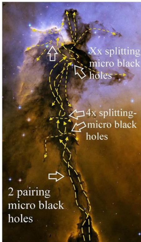
Figure 3, Comparison with splitting and pairing Micro black holes inside Planetary nebula ( Eagle ) , and the formation of comet nuclei like the Hyperion icy nucleus.
