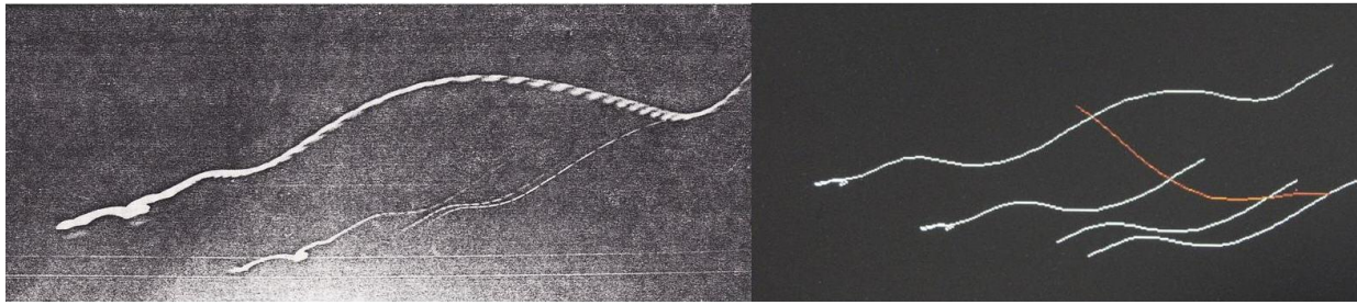
Figure 5, Example of micro black hole production possibly by strong electromagnetic or x-ray interference at sea level. There are four traces to be observed with comparable waveforms. ( see also at the right side: reconstruction image). The left photo is made by Mr. Overhagen (the Netherlands) by automatic shutter camera through his roof window, during heavy thunder storm. The two bumps at the end of two waveforms could be the start of the formation of a micro Black hole.
