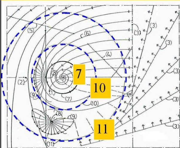
Figure: 21, Electric Black Hole based Comets and Micro comets.
