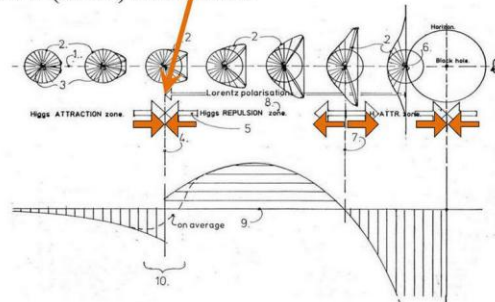
Figure 3, Comparison with splitting and pairing Micro black holes inside Planetary nebula ( Eagle ) , and the formation of comet nuclei like the Hyperion icy nucleus.
