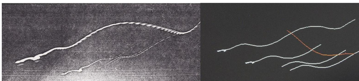
Figure 4, Example of micro black hole production possibly by strong electromagnetic or x-ray interference at sea level. There are four traces to be observed with comparable waveforms. ( see also at the right side: reconstruction image). The left photo is made by Mr. Overhagen (the Netherlands) by automatic shutter camera through his roof window, during heavy thunder storm. The two bumps at the end of two waveforms could be the start of the formation of a micro Black hole.
