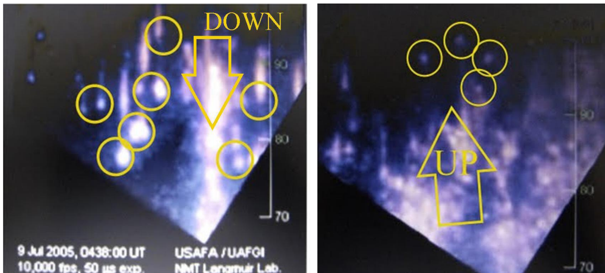
Figure 2, FIREBALL images observed inside a Sprite by a video. The video is made by a High speed camera (10.000 f/sec) of the Langmuir laboratory (USA, 2005) looking at 70-120 km altitude.
