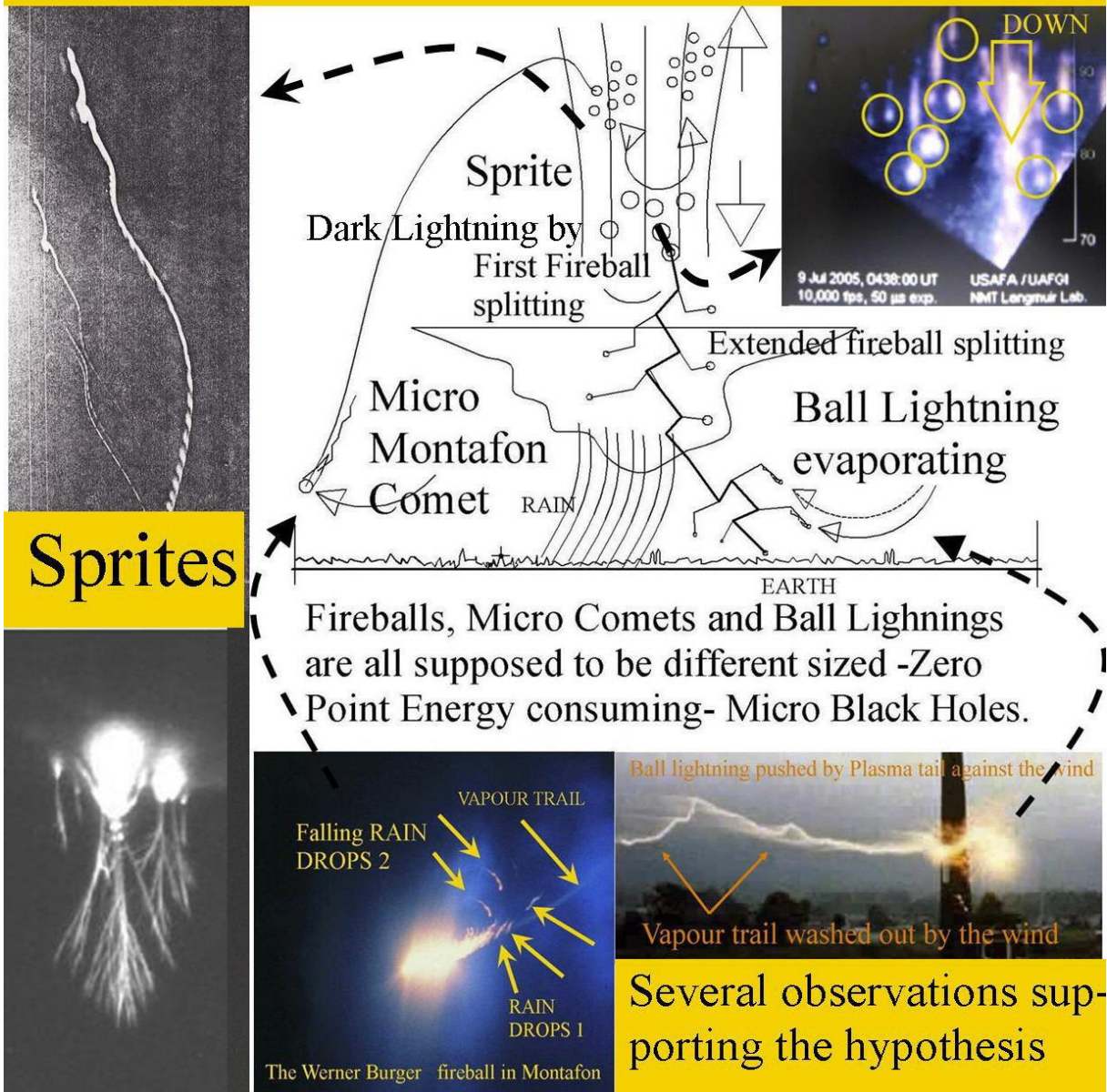
Figure: 13, Several examples of Quantum Knot Ball Lightning created by electro magnetic Interference, Micro Comets and Sprite fireballs combined with Gamma ray "Dark lightning".
