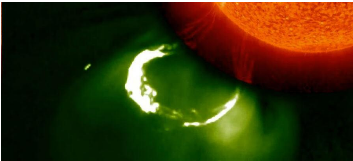
Figure: 16, Fireball production of the sun, leading to micro Comets comparable to Sprite fireballs on earth .
