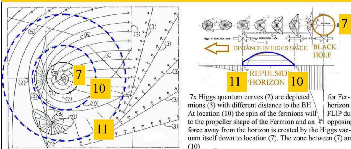
Figure: 21, Electric Black Hole based Comets and Micro comets.
