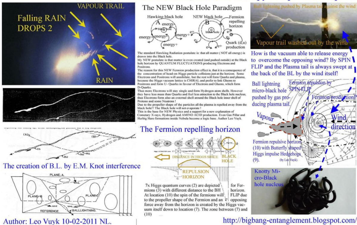
Figure 15, The start of my research was: Ball Lightning physics. Such as Quantum Knot-interference BLs and the origin of acceleration of Knotty BL micro black holes (Quantum Knots) by pushing plasma tails.
