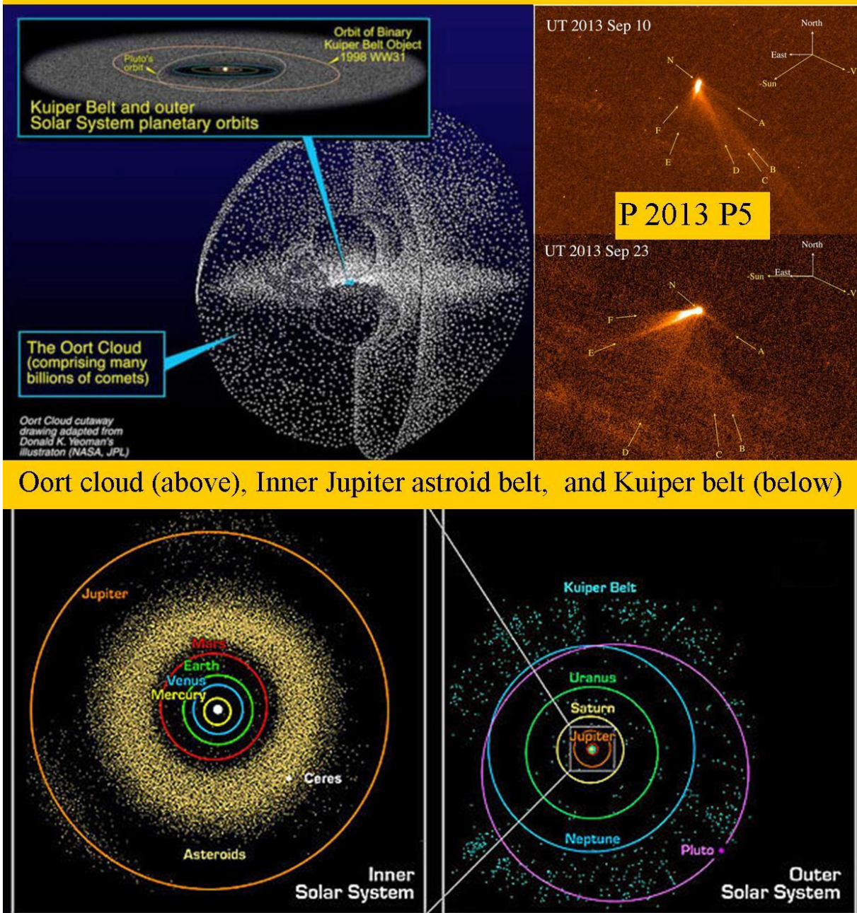
Figure: 18, The solar baby comets are supposed to travel onto the different clouds or belts like the Oort cloud and Kuiper- and Inner Jupiter belt.
