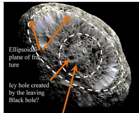
Figure 9 , Principle of the new black hole paradigm All Fermions going OUT only dark energy of the oscillating Vacuum lattice frame is going IN..
