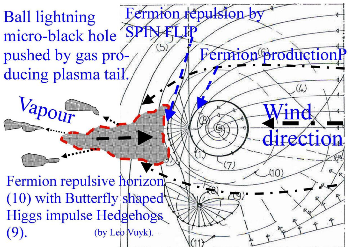
Figure 6, It is assumed that the New Paradigm Black hole is able to use and accumulate so called "Zero Point Energy" to form Plasma tails which seem to be able to push the black hole away from the centre of mass of the earth. (Ref. 4 )
