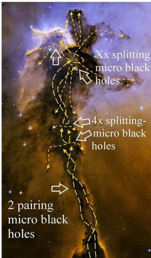
Figure 10 , Comparison with splitting and pairing Micro black holes inside Planetary nebula ( Eagle ) , and the formation of comet nuclei like the Hyperion icy nucleus.
