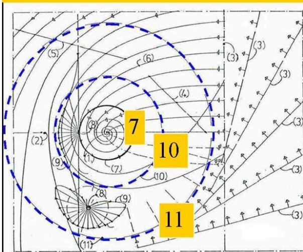
Figure: 20, Electric Black Hole based Ball Lightning
