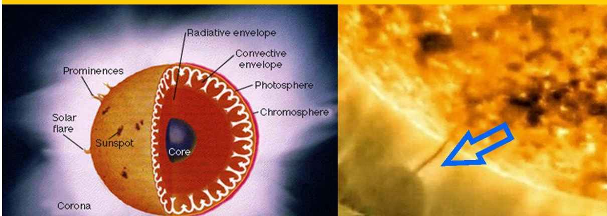
Figure: 17, ( see also ref. [13]) Bright points or spots at the solar surface represent small Comets able to leave the sun by new pushing Cometary tails like Ball Lightnings do. The origin of these bright points are supposed to be so called “Interference black holes” according to Q-FFF theory.
