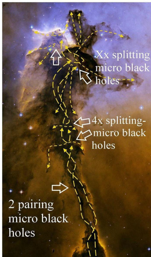
Figure 9, Principle of the new black hole paradigm.
