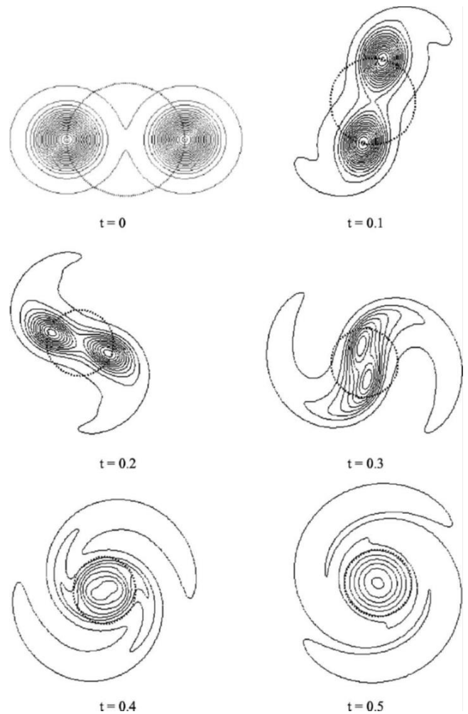
Fig. 4. Time evolution of the vorticity contours during the merging process of two equal co-rotating vortices with equal angular velocities. A circle with constant diameter is plotted for reference. Figure from Huang’s article above mentioned, used by permission.
