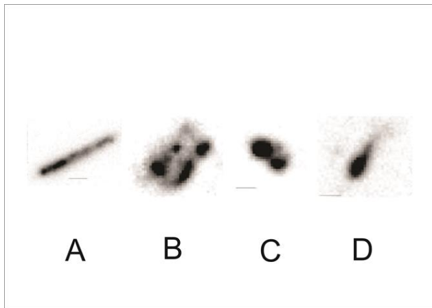
Fig. 1. Odd shaped galaxies at very high redshifts from the Hubble Ultra Deep Field galaxy survey. A is a chain galaxy, B is a clump-cluster, C is a double clump and D is a tadpole.
