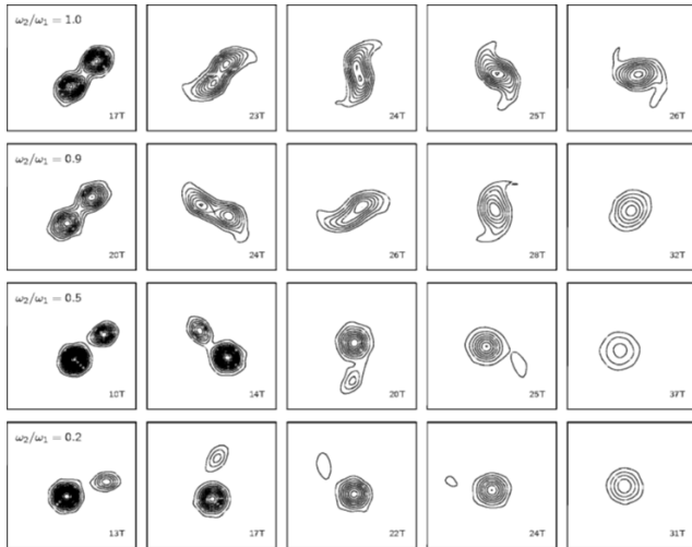
Fig. 6. Mergers of two vortices with equal and different angular speeds. It corresponds to Fig. 16 in the paper by Trieling et al. [110]. Figure used by permission.
