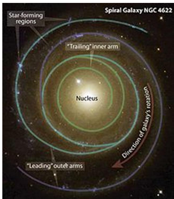
Fig. 8. NGC 4622 looks like a modified Lundgren's spiral vortex and, therefore, should have been formed by the merger of a large vorteeon with 3 small vortees, one in co-rotation with the large vorteeon and the other two in counter-rotation with the large vorteeon. Picture from Wikipedia.
