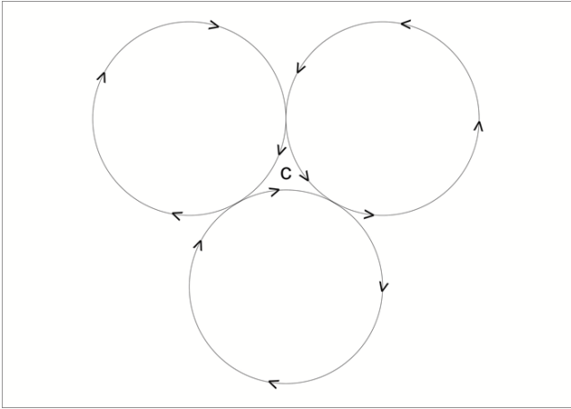
Fig. 9. In the region C among the rotating clusters there are fast and slow vortons whose mergers generate elliptical galaxies.
