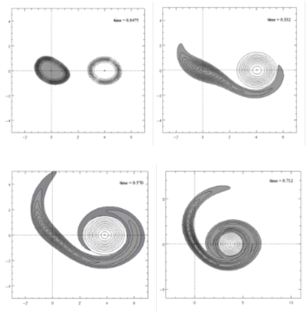
Fig. 7. Illustration of some steps of the time evolution of an asymmetric merger of two vortices. It is part of Fig. 1 of reference [114], used by permission.
