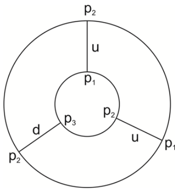
Fig. 2. Pictorial representation of the arrangement of primons in the proton. In the neutron the inner layer is the same, and in the outer layer the p_1 below is replaced by p_3 and this makes the neutron to be udd in terms of quarks.
