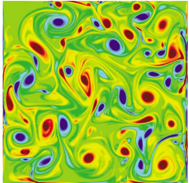
Fig. 3. How the vortons and the fluid of nucleons and electrons inside each cluster of galaxies will look like after galaxies lose their outskirts due to the shrinking of the cluster by its gravity. Galaxies will be reduced to rotating spheroids of nucleons, which we may call vortons. In this figure the vortons are the roundish blue and red bodies. The figure is from an article by Clercx et al. [87] on turbulence in two dimensions in square and circular domains (figure used by permission).
