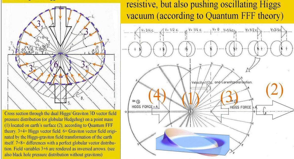
Figure 20, equivalence between gravity and acceleration does not hold in Q-FFF theory.
