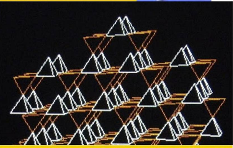
Truncated tetrahedron space according to the Quantum-FFF model. Each tetrahedron lattice has a spiral shape based on three linear units
