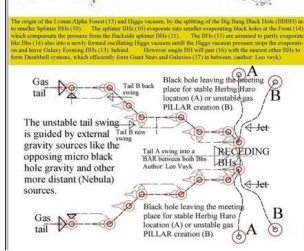
Figure 24, star formation and dying according to Quantum-FFF Theory.
