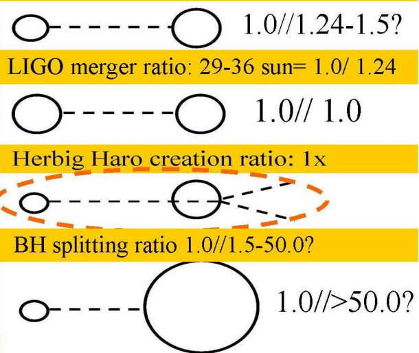
Figure 9, suggestions for black hole nuclear splitting and merging by BH nuclear collision of different sizes.
