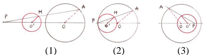
F.5. \rightarrow For any point A on , and P Out-On-In circle [O, OA] and O'P = O'O , exists O'M = OA / 2 .
