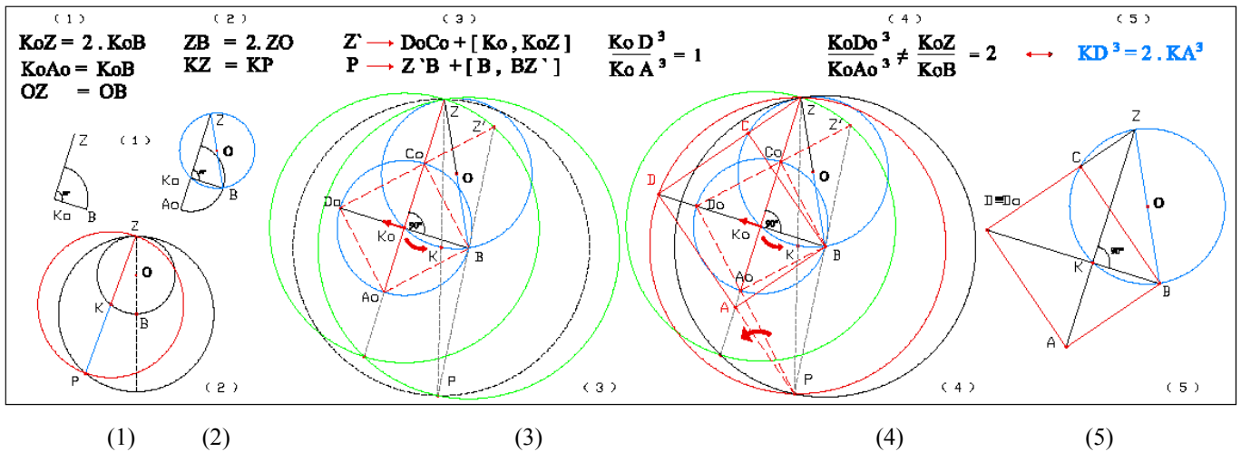
F.4.. \rightarrow The Mechanical Extrema Constant Poles of rotation in any circumcircle of triangle ZKOB .
