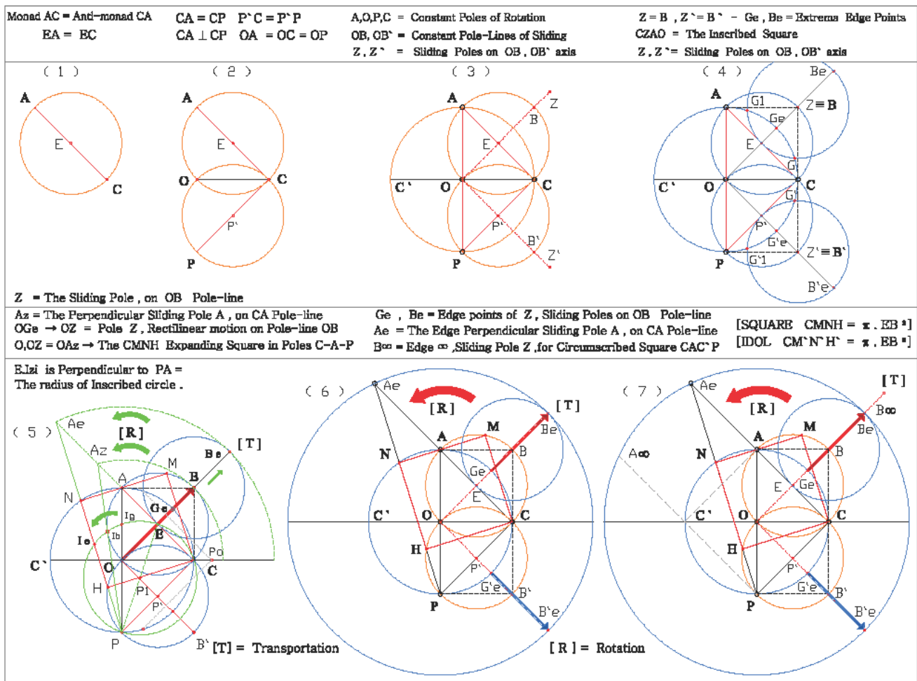
F.2 \rightarrow The steps for Squaring the circle ( E, EA = EC ) on diameter CA through Plane Procedure Mechanism.
