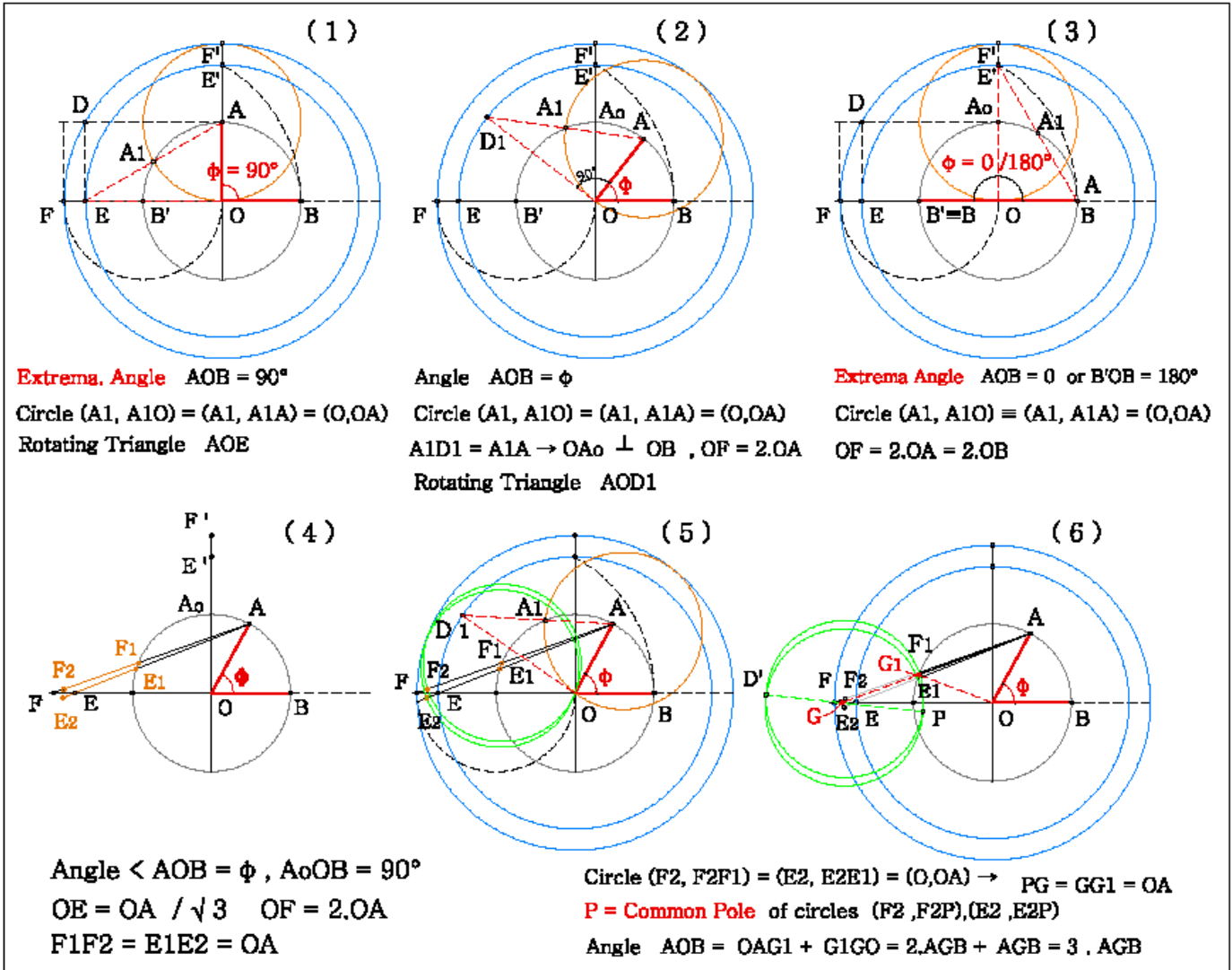
F. 11 → The extrema Geometrical method of the Trisection of any angle \phi < AOB
