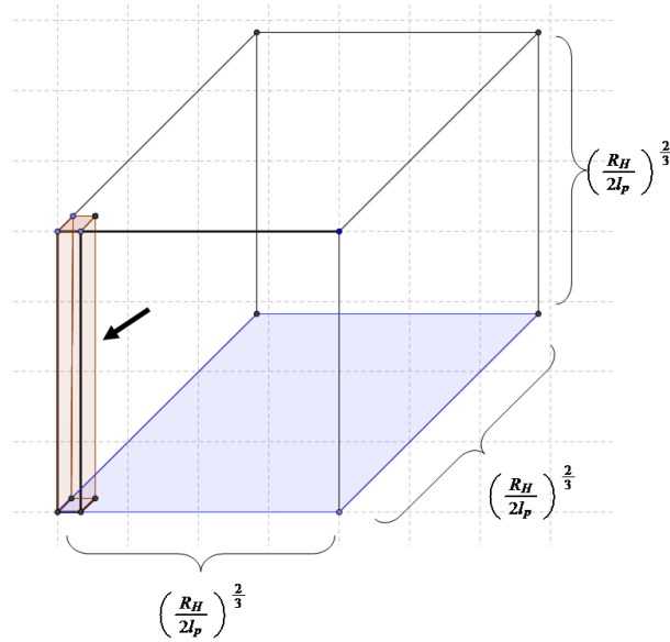
Figure 1. The large number cube. The length of each side of the cube is equal to the cube root of the large number. The square at the very bottom, shown in blue, represents the
