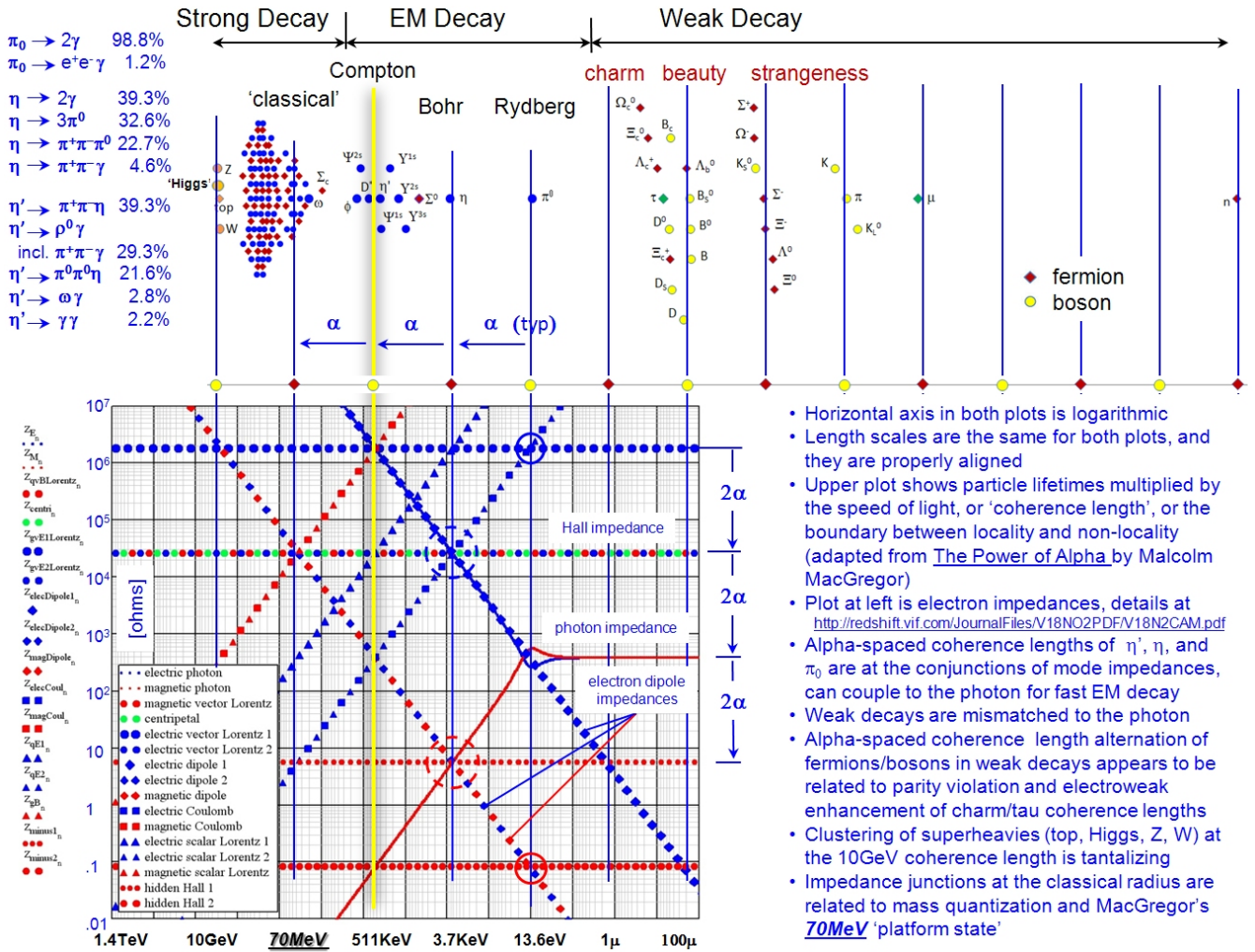
FIG. 2. A composite of 13.6eV photon impedances and a variety of electron impedances [5, 6], measured branching ratios of the \pi_0 , \eta , and \eta' , the four fundamental quantum lengths shown in fig.1, and the coherence lengths of the unstable particles. Regarding dipole impedances, only the transverse dipole-dipole impedances are shown. Missing are the longitudinal dipole-dipole and longitudinal and transverse charge-dipole impedances.
